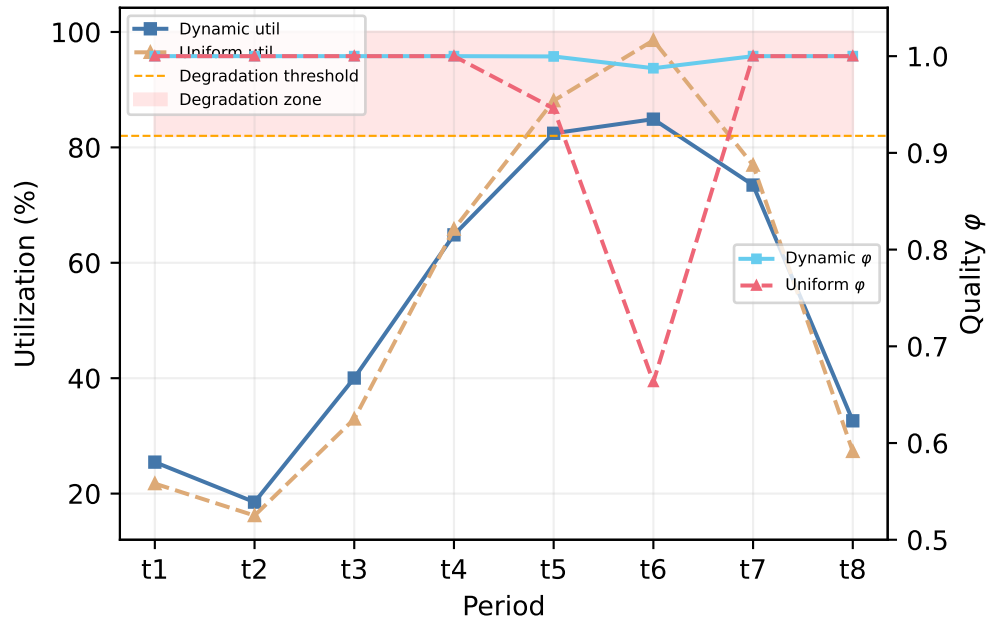
Utilization & Service Quality
