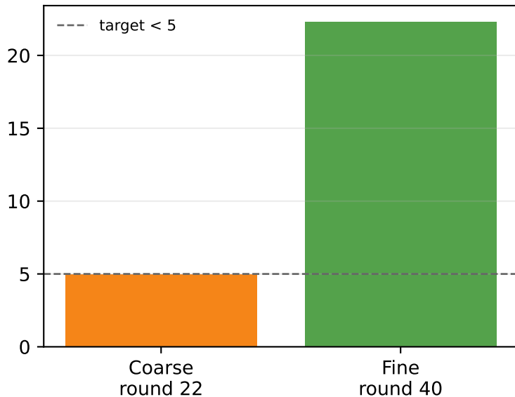
Final stored max regret
