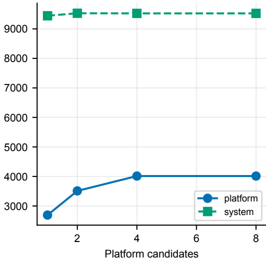
Best objective
