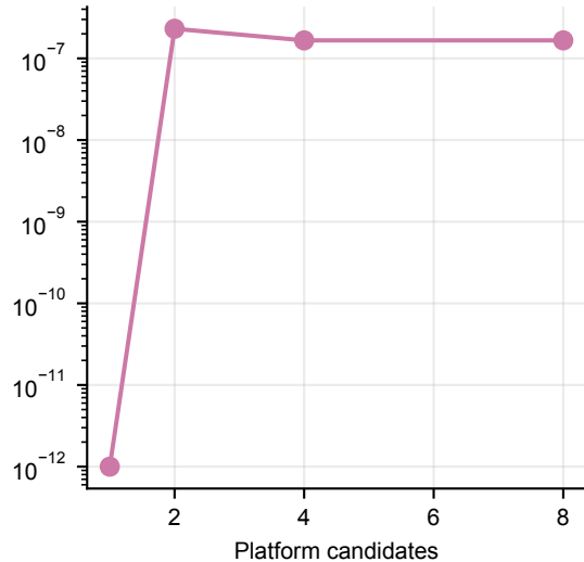
Regret diagnostic
