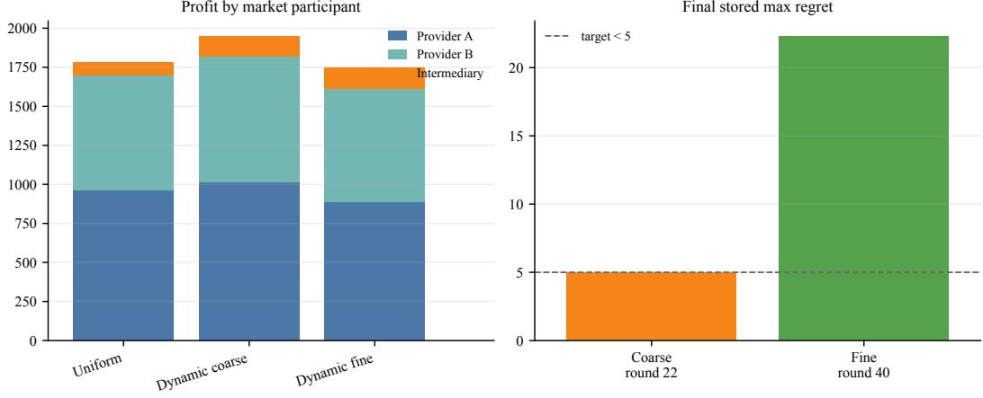
Figure 4: Profit components and pure-strategy regret boundary. The left panel decomposes profit by market participant, and the right panel reports stored best-response regret. The coarse snapshot reaches regret < 5 , whereas the fine-grid pure snapshot remains at 22.3 and is used only as a resolution stress test.
