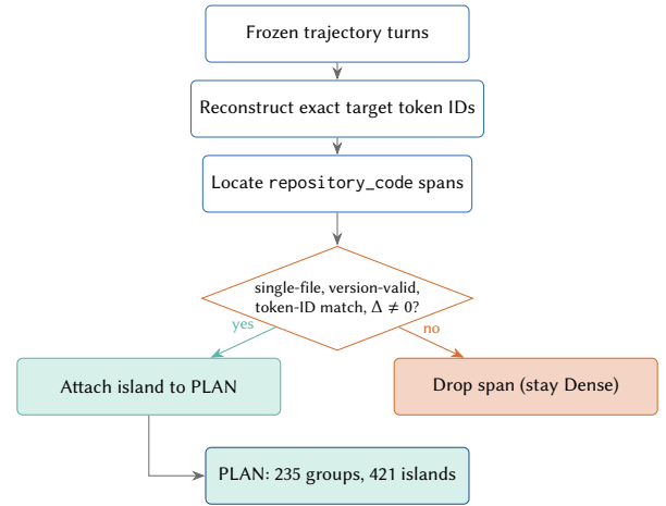
Offline oracle on frozen traces; not an LLM-synthesized DAG.
