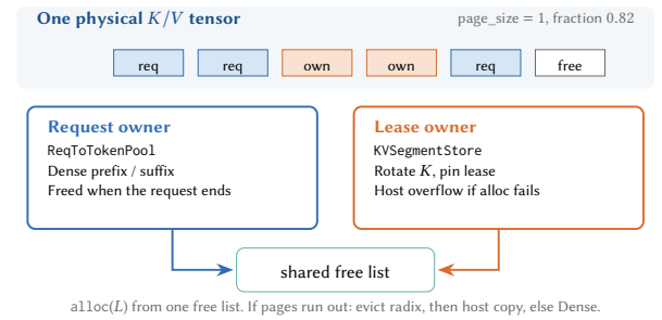
Figure 12. One physical KV pool, two owners. Request slots hold Dense prefix/suffix; leased slots hold admitted islands. Allocation is dynamic; the engine does not reserve a fixed island fraction.
