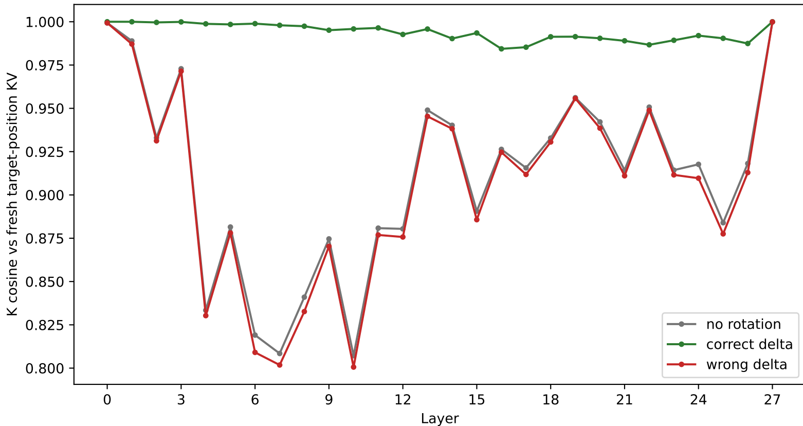
Layer-wise key alignment for an AST-selected exact span
