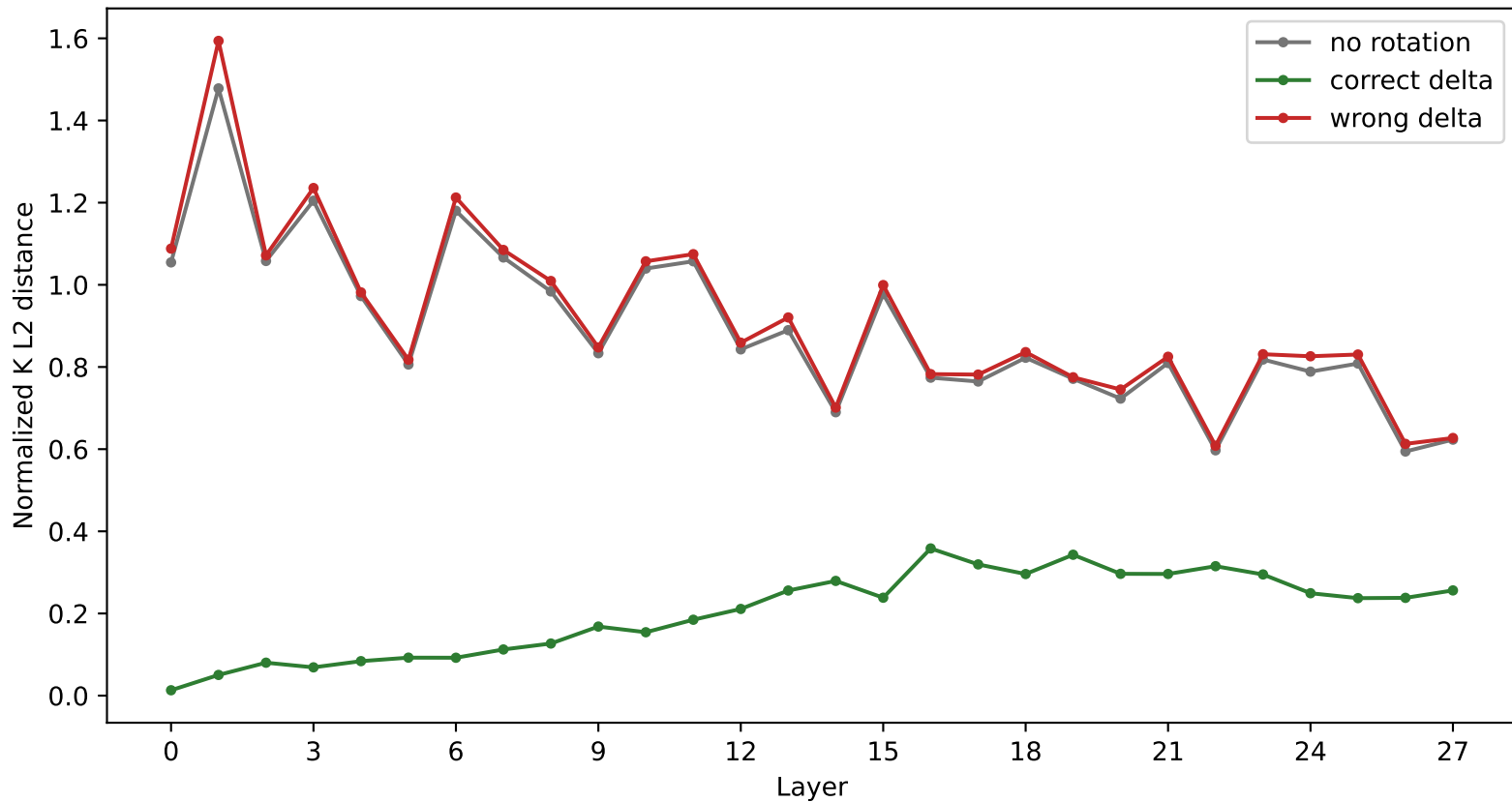
RoPE delta reduces layer-wise key distance
