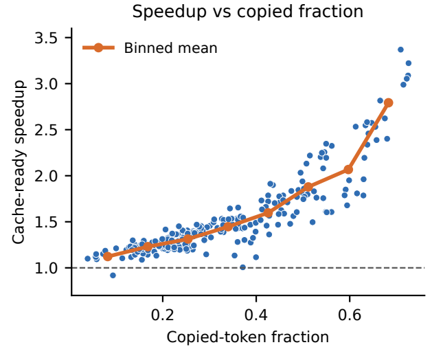
Figure 14. Per-group cache-ready speedup versus copied-token fraction, with a binned-mean line. Groups that copy more of the prompt are faster; the headline 1.492× is not a short-prompt artifact.
