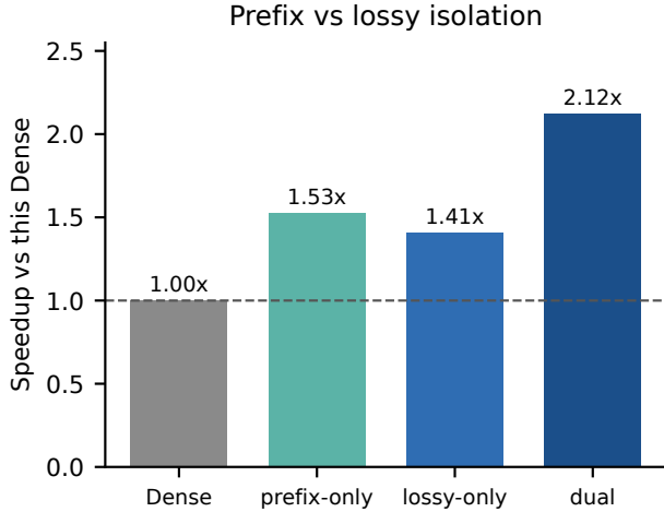
Figure 15. Prefix-on isolation on the 235-group PLAN (job 139839). Dual is copy plus radix, not a prefetch win. Not Table 5.
