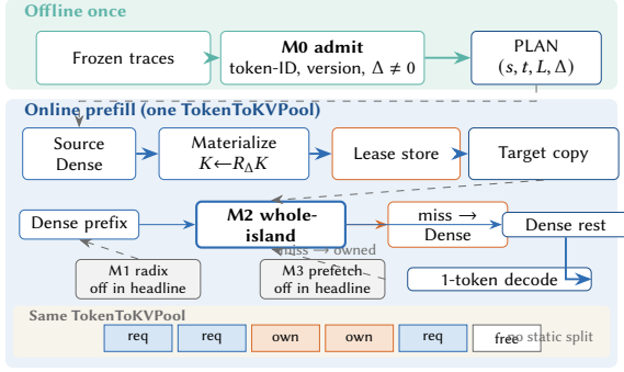
Figure 8. System design. M0 compiles a PLAN offline. Online prefill uses one TokenToKVPool: request slots for Dense spans, leased slots for admitted islands. Headline 7B speed is M0+M2; M1 and M3 stay off so Table 5 cannot be credited to radix or prefetch.
