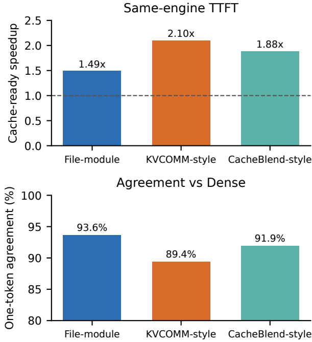
Figure 16. Same-engine admit clones (job 137400). Unconstrained copy is faster and agrees less. Not native CacheBlend/KVCOMM stacks and not Table 5.
