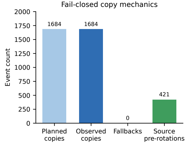
Figure 19. Fail-closed copy mechanics (job 137185). 1684/1684 planned copies, 0 fallbacks, 421 source K pre-rotations. Not mixed into Table 5.
