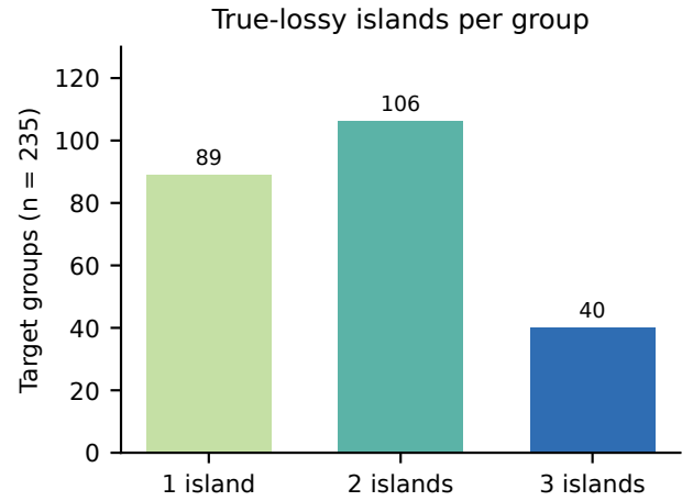
Figure 20. True-lossy islands per target group on the 7B PLAN ( n=235 ). Not a new GPU arm and not Table 5.
