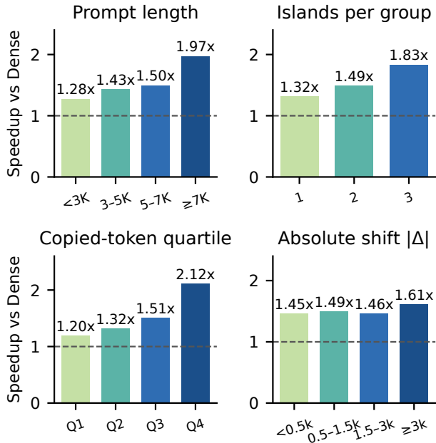
Figure 17. Cache-ready TTFT speedup on the same 705 pairs (job 137185). Not a new GPU arm and not Table 5.
