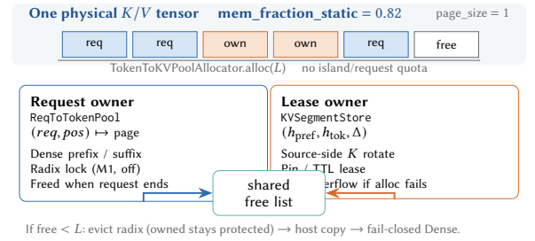
Figure 12. One physical KV pool, two owners. Request slots hold Dense prefix/suffix; leased slots hold admitted islands. Allocation is dynamic; the engine does not reserve a fixed island fraction.
