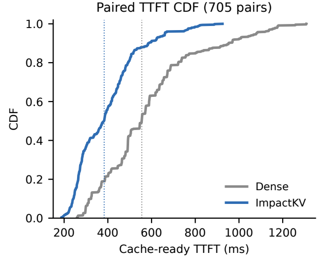
Figure 13. Empirical CDF of paired cache-ready TTFT (705 pairs, job 137185). ImpactKV shifts the body and the tail: median 555→383 ms, p90 952→586 ms, p99 1178→819 ms.
