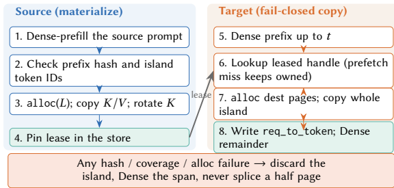
Figure 11. M2 algorithm. Source materializes a leased island with source-side K rotation. Target Dense-computes the prefix, copies the whole island or Densifies it, then Dense-computes the remainder. Mechanical failure never splices a half page.
