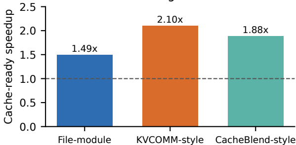
Same-engine TTFT
