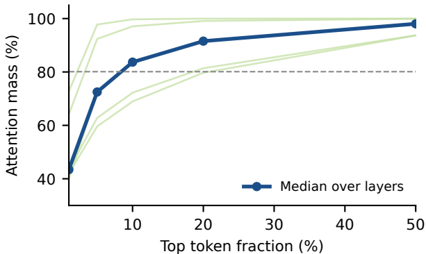
Dense attention sparsity (3B)
