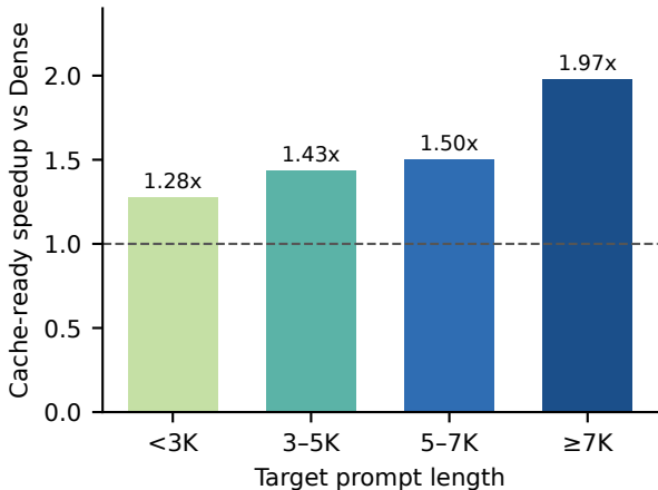
Cache-ready TTFT by prompt length
