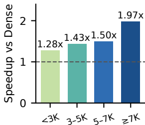
Prompt length
