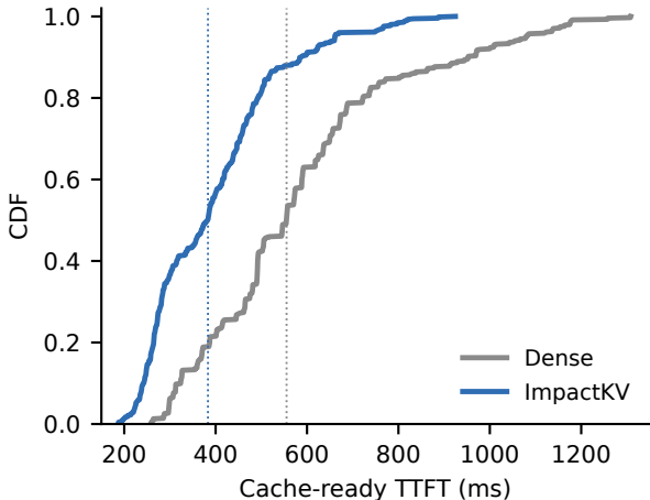
Paired TTFT CDF (705 pairs)
