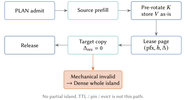
Figure 18. KV object lifecycle. A leased island is either copied in full or discarded; there is no partial serve.
