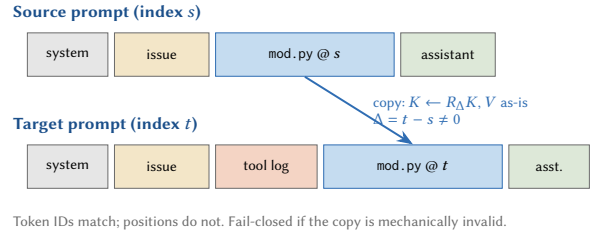
Figure 10. Cross-turn file-module reuse. Token IDs match; positions do not ( \Delta = t - s \neq 0 ). Only K is phase-corrected; V is copied as-is.
