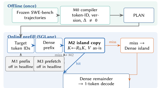
Figure 8. Engine stack for shifted file-module prefill. Online path is Dense prefix, then M2 copy, then Dense remainder. Headline 7B speed uses M0+M2; M1 and M3 stay off so Table 5 cannot be credited to radix or prefetch.
