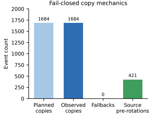
Figure 16. Fail-closed copy mechanics (job 137185). 1684/1684 planned copies, 0 fallbacks, 421 source K pre-rotations. Not mixed into Table 5.
