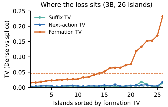
Figure 3. Per-island attention TV after a file-island splice (Qwen2.5-Coder-3B, 26 islands, sorted by formation TV). Suffix attention does not collapse; formation TV is an order of magnitude larger (frozen medians 0.00264 / 0.00492 / 0.0462). Not 30B native and not Table 5.
