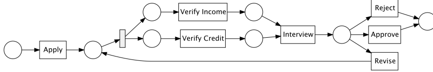
Fig. 1. A perfectly fitting Petri net with the underlying log.
