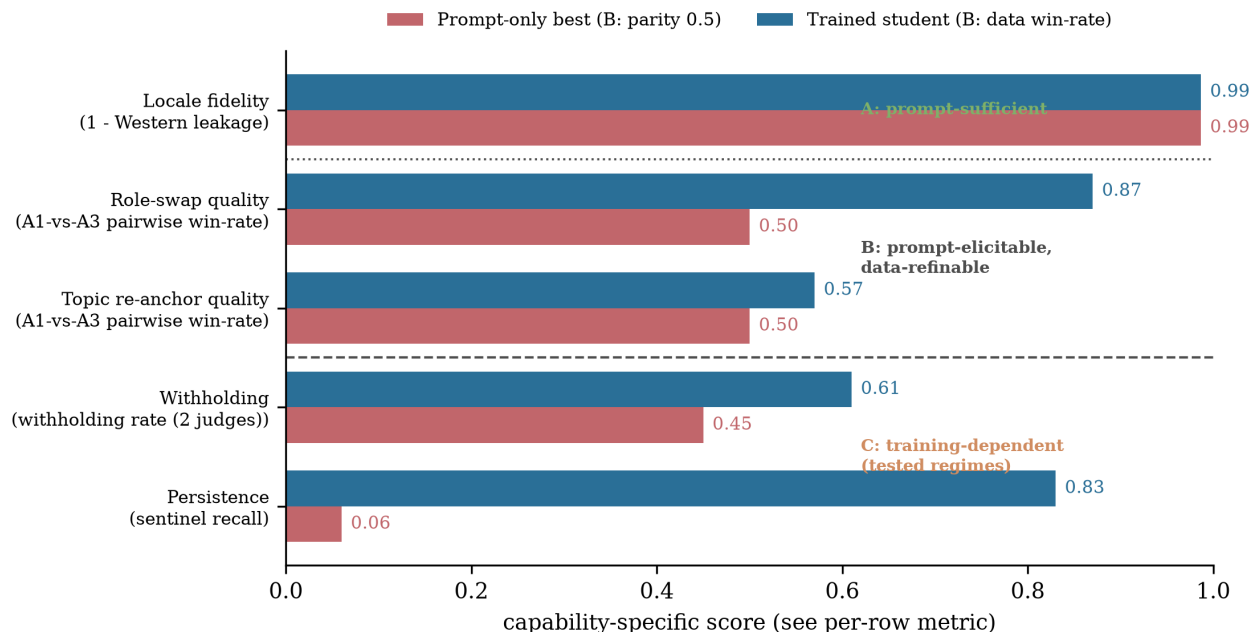
Figure 3: Three regimes of the train-versus-prompt boundary. Each capability is scored by its own validated, capability-specific metric (no heterogeneous metrics are combined on one axis, and the retired context-blind axis-F1 is not used here; §5.5). Regime A (prompt-sufficient) : locale fidelity — prompt-only reaches parity. Regime B (prompt-elicitable but data-refinable) : role-swap and topic re-anchoring — the behavior type appears prompt-only, but specialized data wins the pairwise quality comparison (§5.6). Regime C (training-dependent under the tested regimes) : multi-turn persistence and pedagogical withholding — prompt-only falls far short despite the identical instruction. Persistence prompt-only is the 9B teacher’s zero/few-shot recall ( \leq 0.06 ); withholding prompt-only is the 9B teacher (0.45). Interval estimates and full statistics in Table 8.
