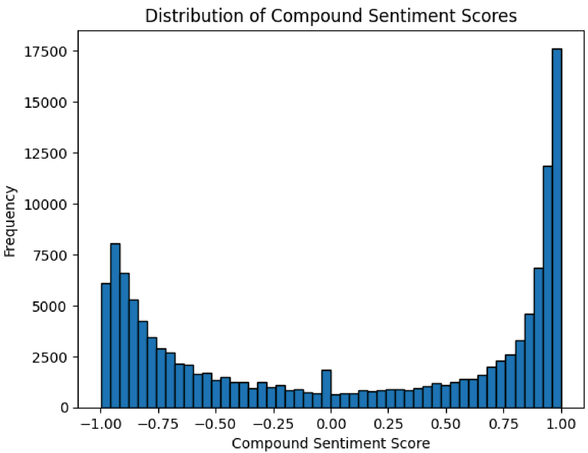
Figure 2: Sentiment Distribution
