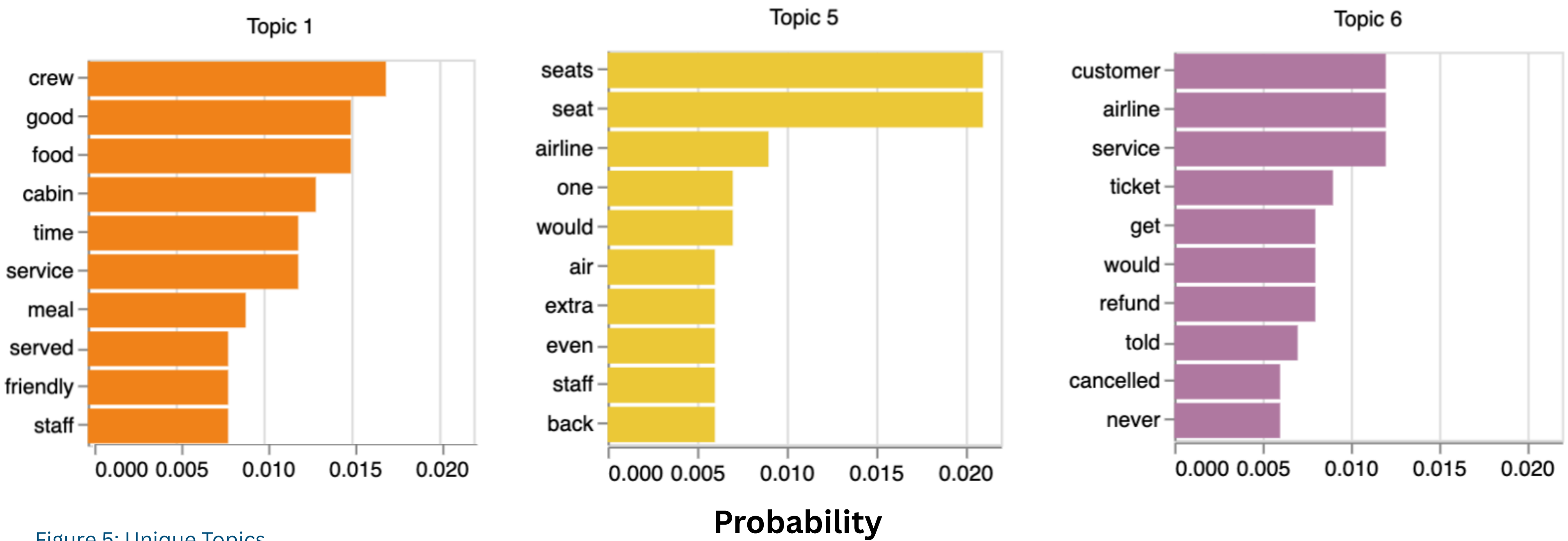
Figure 5: Unique Topics
