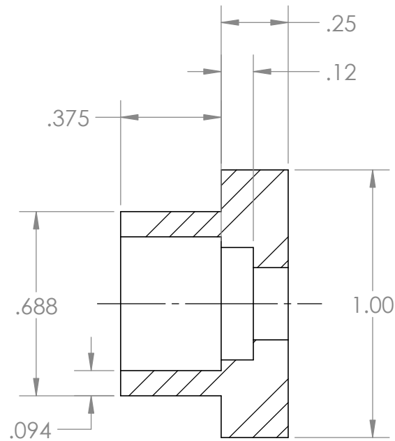
SECTION B-B
