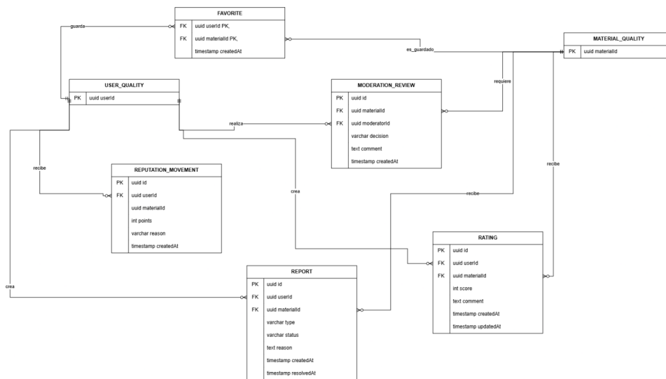
Figura 6: ApuntesUCT - MER Quality Service.
