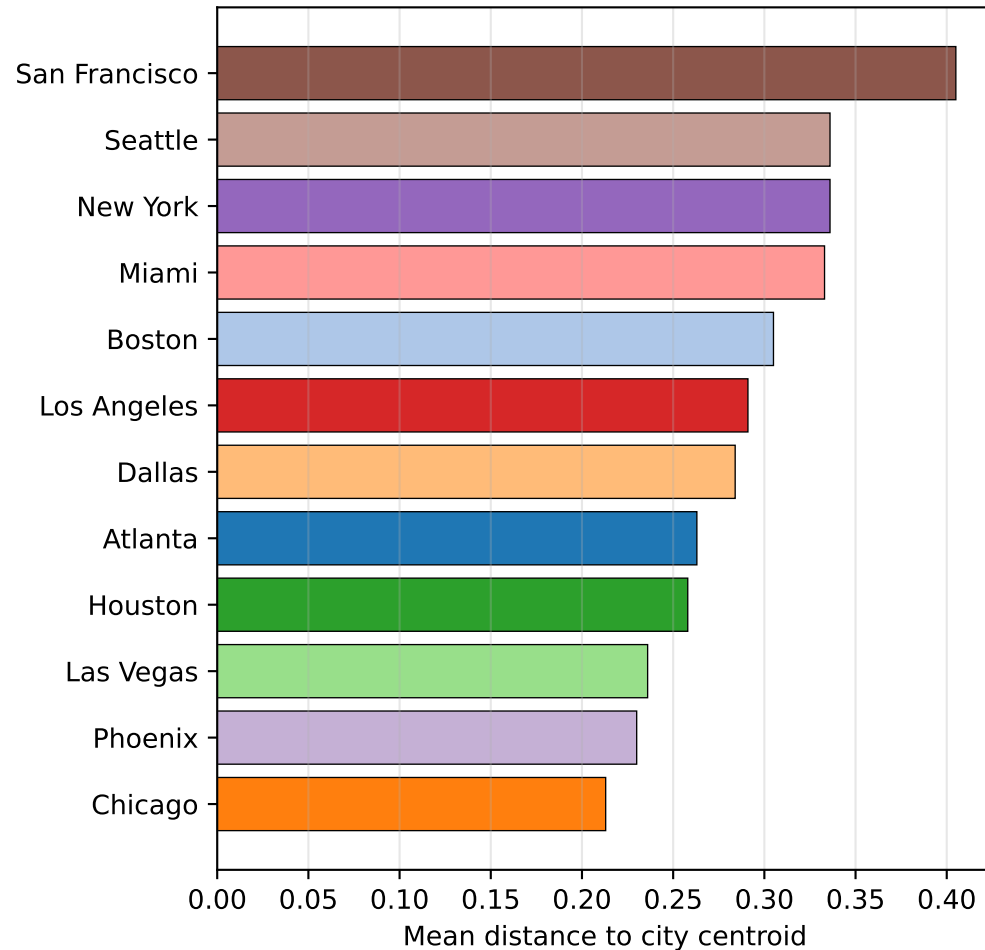
Within-city dispersion (heterogeneous → PERMDISP sig.)
