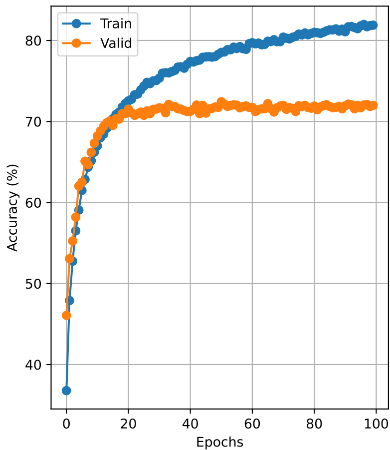
Without augmentation Test Acc: 71.090
