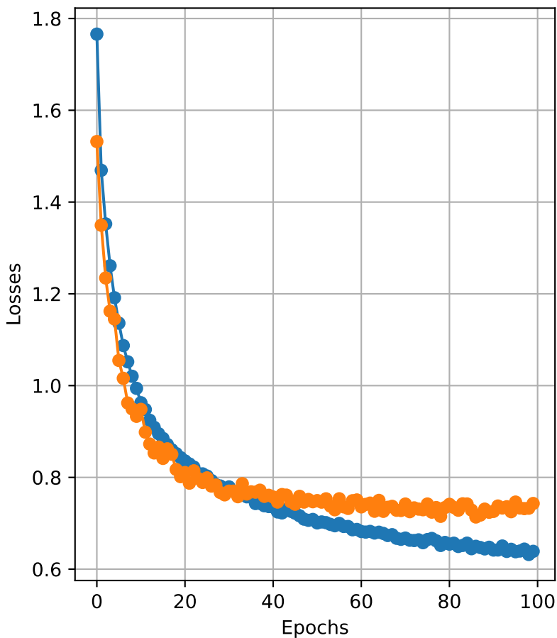
Without augmentation Test Loss: 0.906
