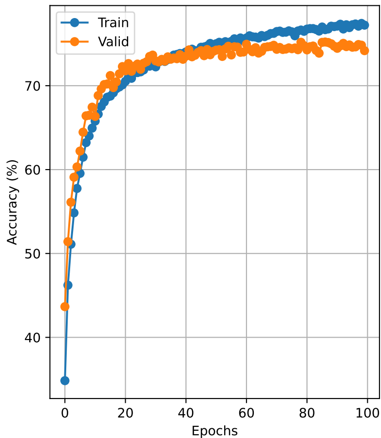
Without augmentation Test Acc: 71.090
