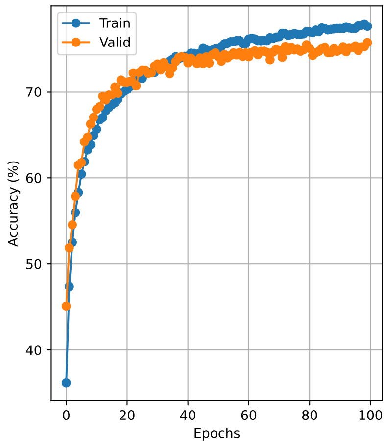
Without Batch norm Test Acc: 75.720
