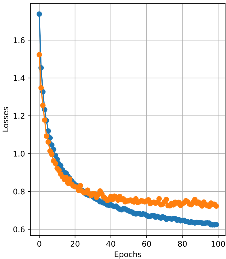
Without Batch norm Test Loss: 0.710
