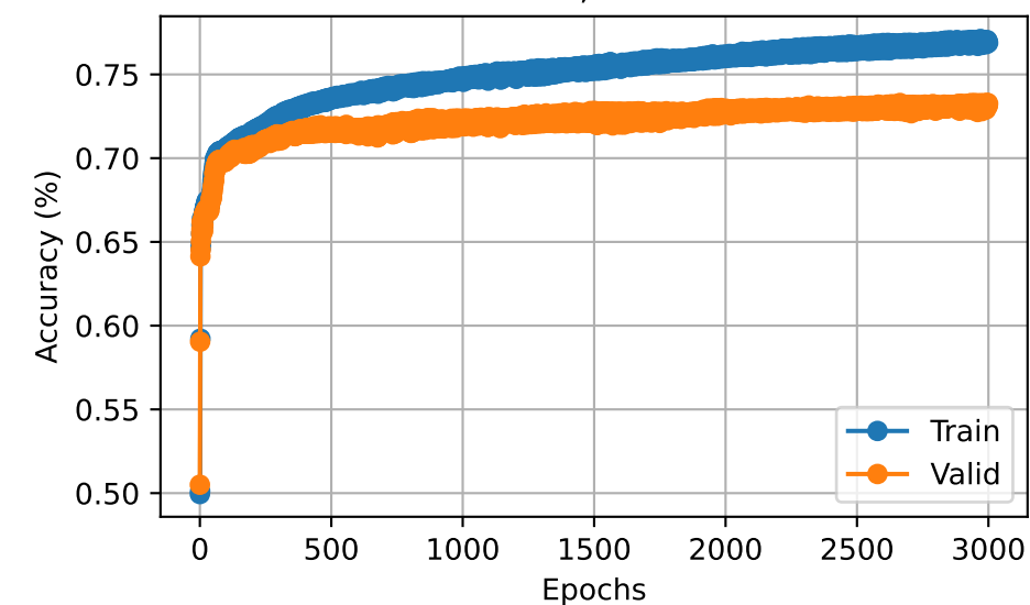
Epochs= 3000, N_{layers} = 4 bias= 0.059, var= 0.0596
