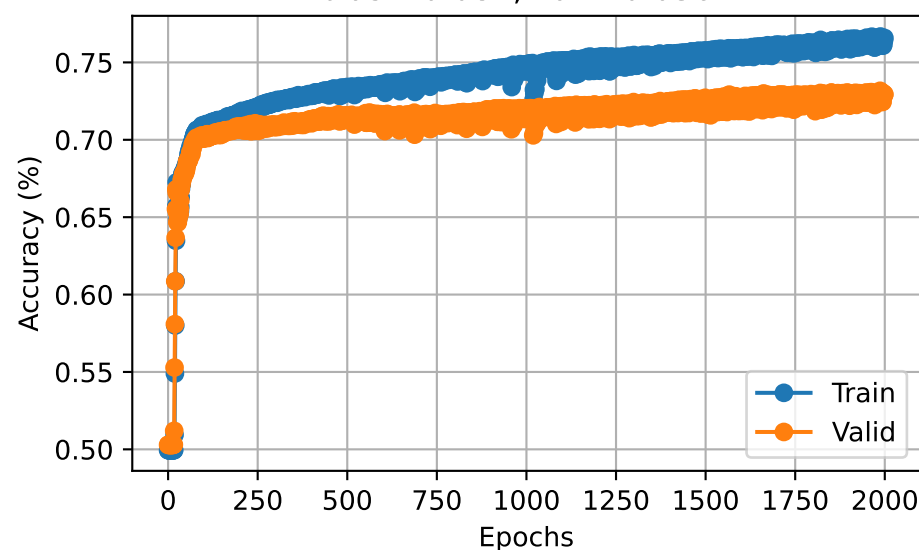
Epochs= 2000, N_{layers} = 5 bias= 0.084, var= 0.0364
