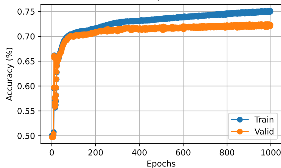
Epochs= 1000, N_{layers} = 4 bias= 0.089, var= 0.0357
