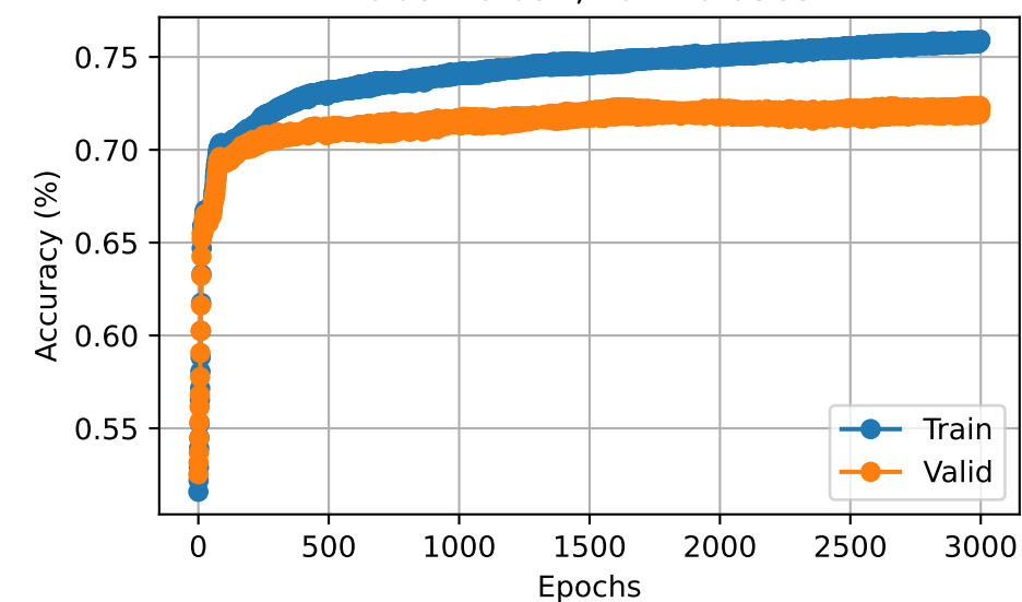
Epochs= 3000, N_{layers} = 3 bias= 0.081, var= 0.0362
