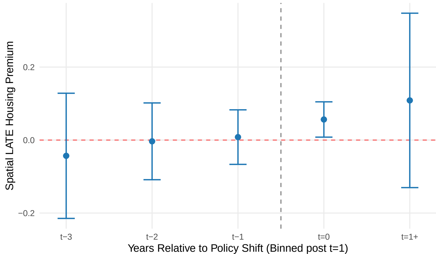
Event Study 3: Binned (L1 absorbs t \geq 1 )
