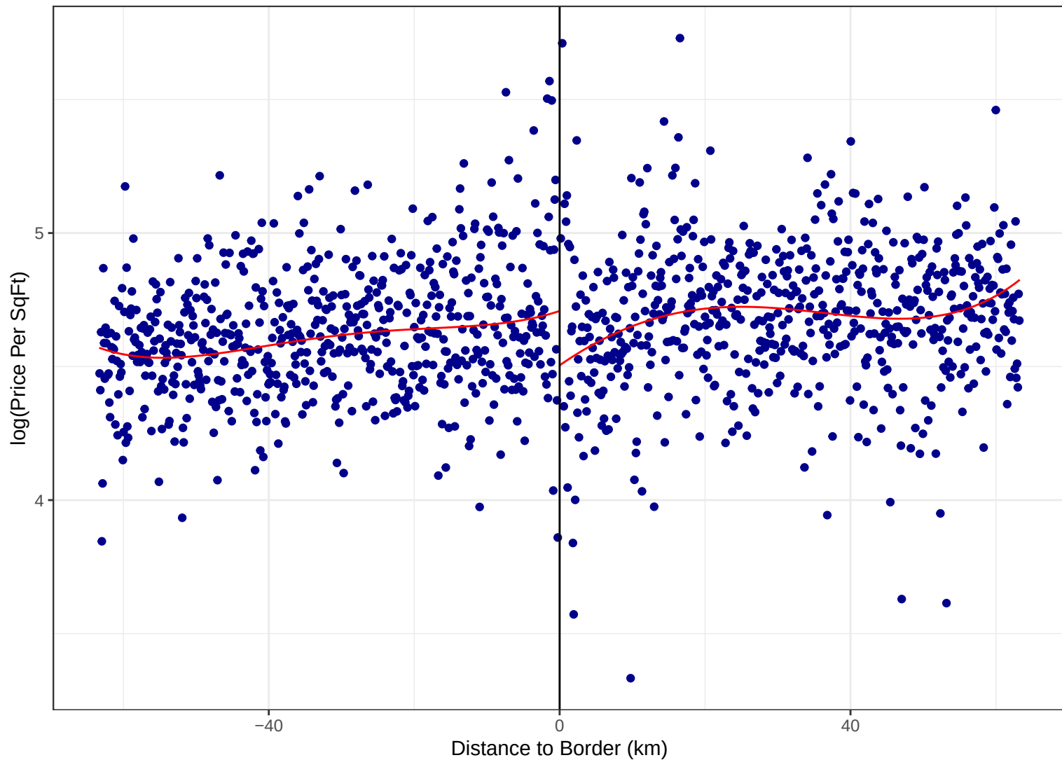
Local Discontinuity: House Price vs. Top 50 Prestige Access
