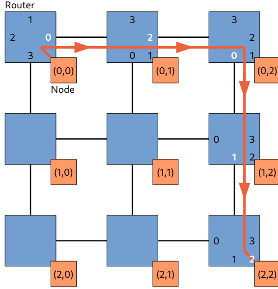
Fig. 8. Relative hop encoding for a 3 \times 3 mesh network.
