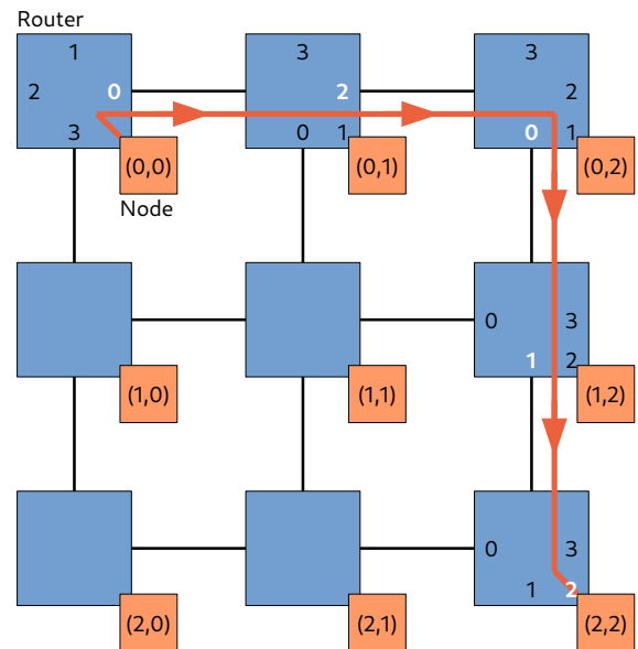
Fig. 8. Relative hop encoding for a 3 \times 3 mesh network.
