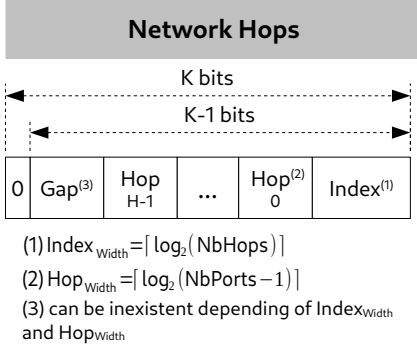
Fig. 10. Network Hops flit structure.
