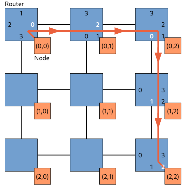
Fig. 11. Relative hop encoding for a 3 \times 3 mesh network built with 5-port routers. The hop list [0 \rightarrow 2 \rightarrow 0 \rightarrow 1 \rightarrow 2] establishes a path from node (0,0) to node (2,2) . Each hop ID is relative to the ingress port: hop 0 denotes the next counterclockwise egress, excluding the ingress port itself.
