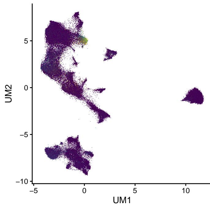
PECAM1 (0–4.7)
