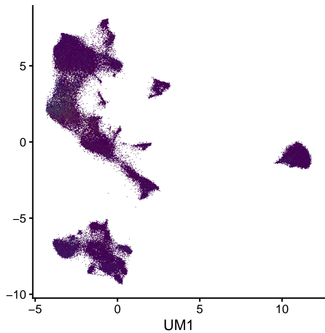
JCHAIN (0–3.1)
