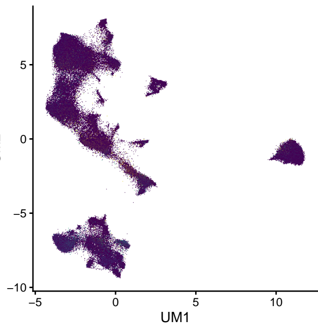
ELANE (0–4.3)
