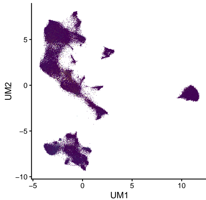
IGHG1 (0–8.2)
