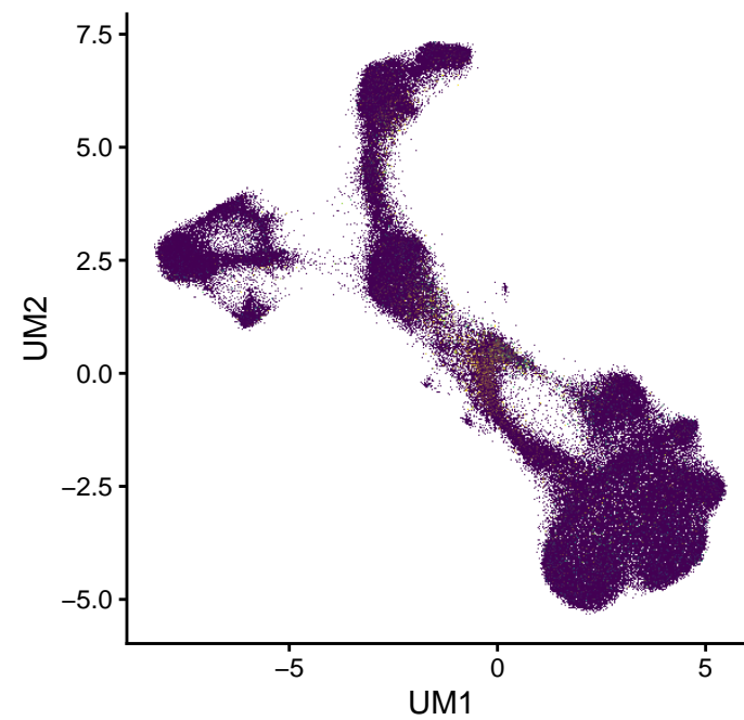
CD2 (0–4.6)
