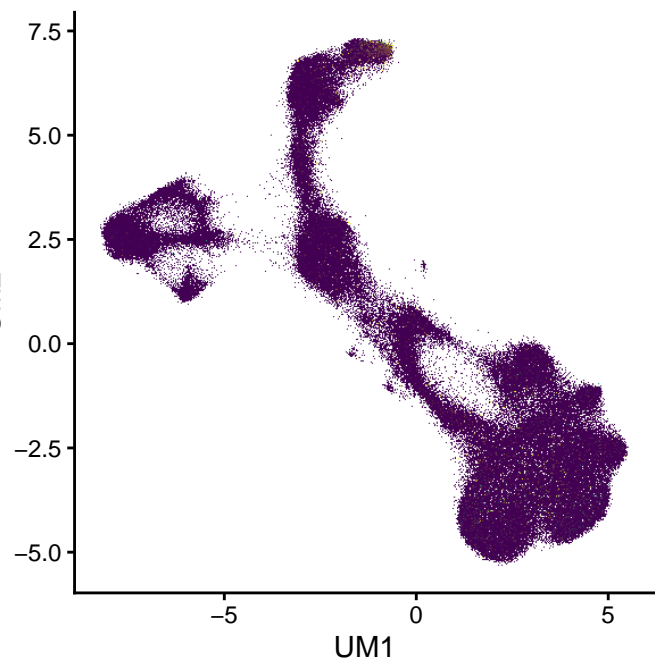
ELANE (0–4.3)
