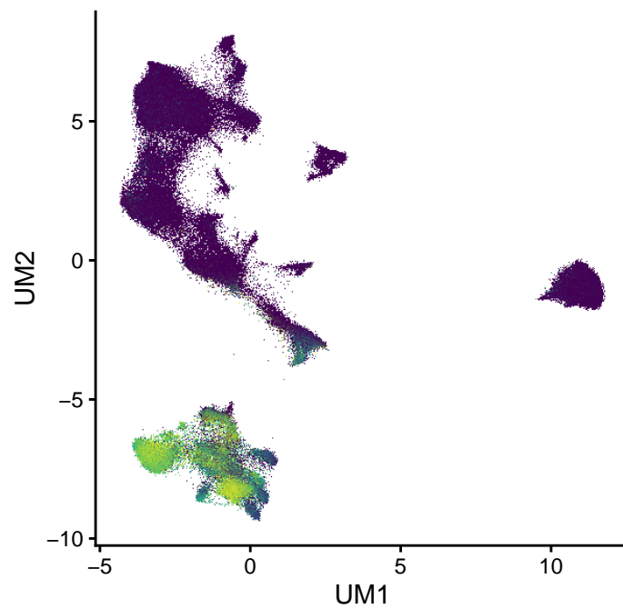
KRT19 (0–5.9)
