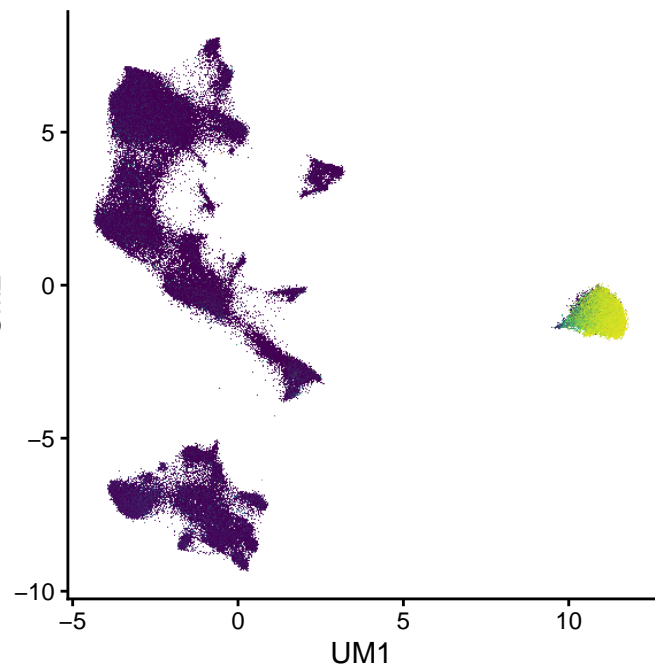
ELANE (0–4.3)
