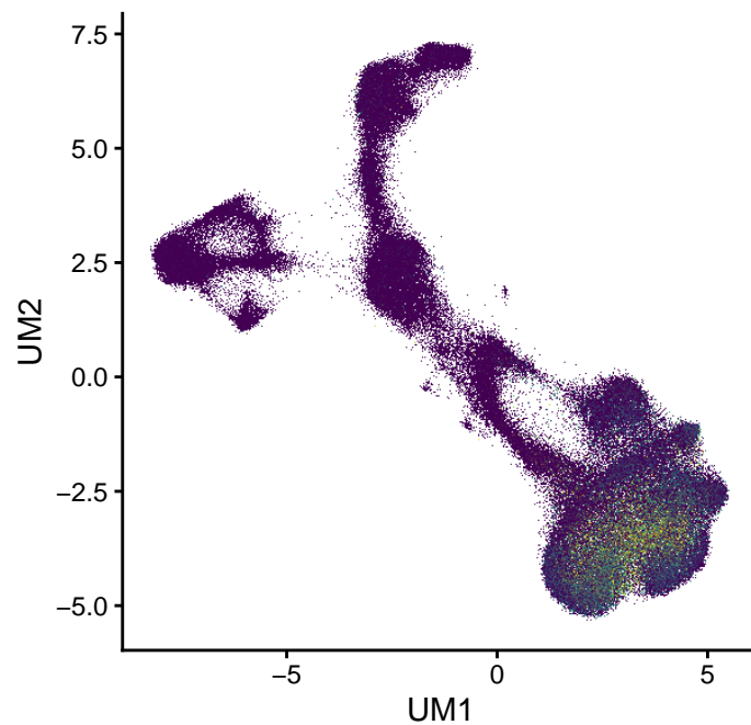
KRT19 (0–6.7)
