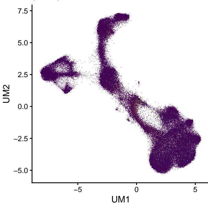
IGHG1 (0–9.4)
