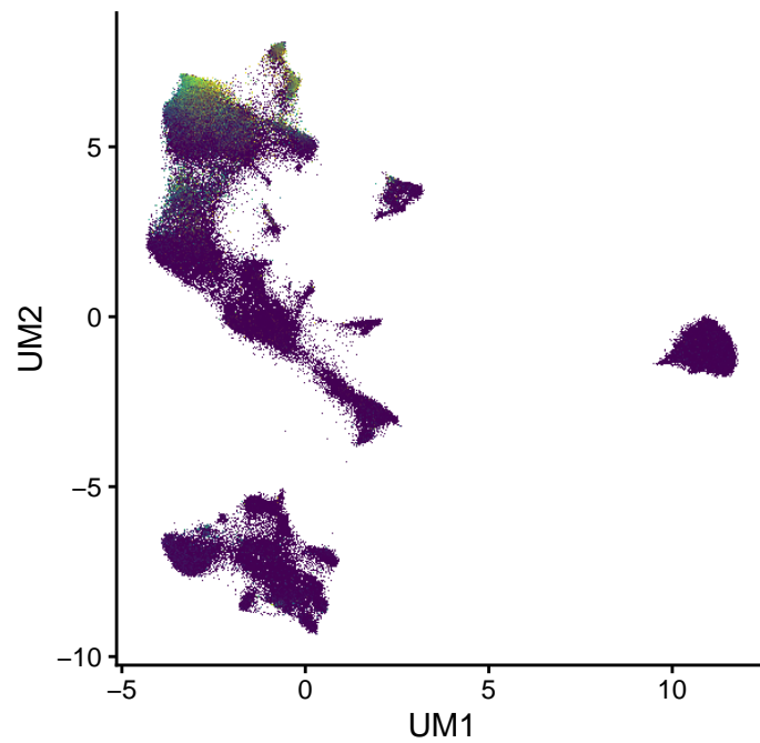
KRT19 (0–5.9)
