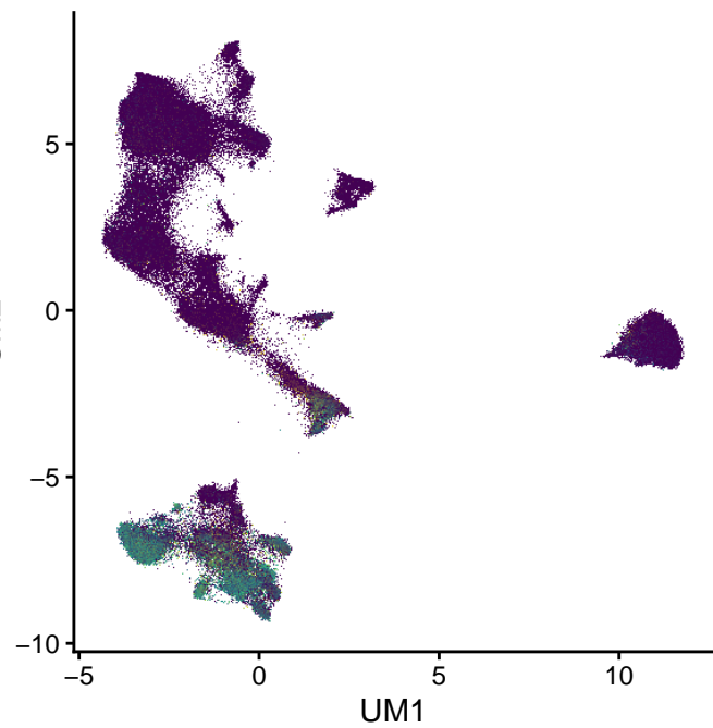
CD74 (0–6.6)
