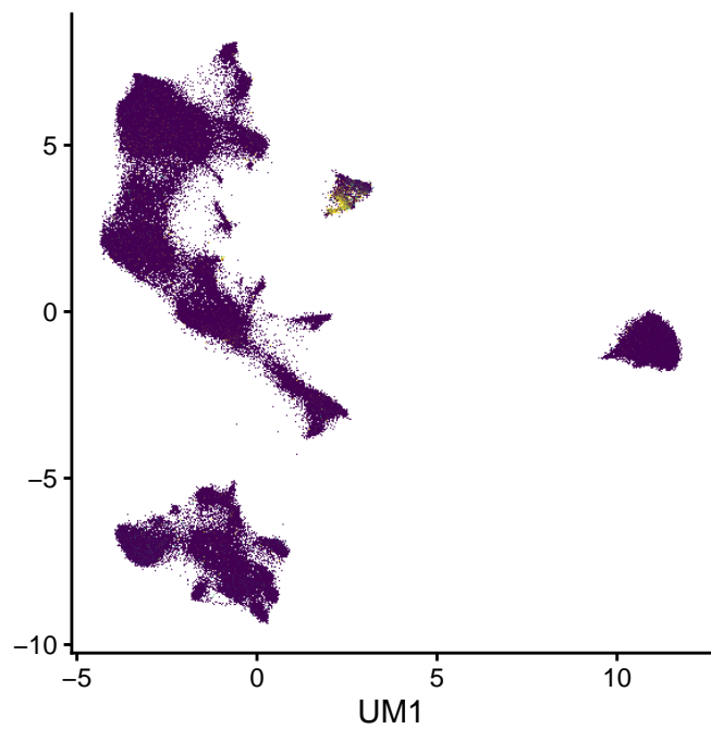
JCHAIN (0–3.1)
