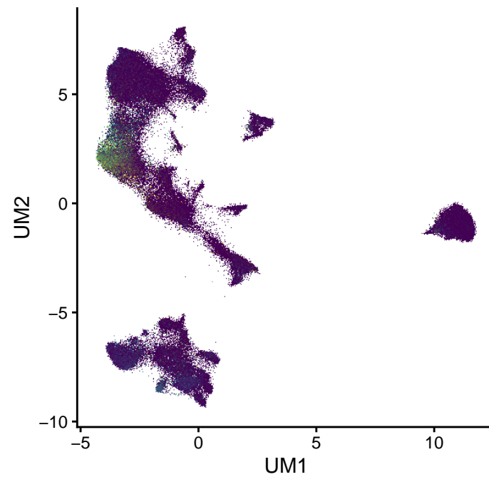
CD2 (0–3.6)
