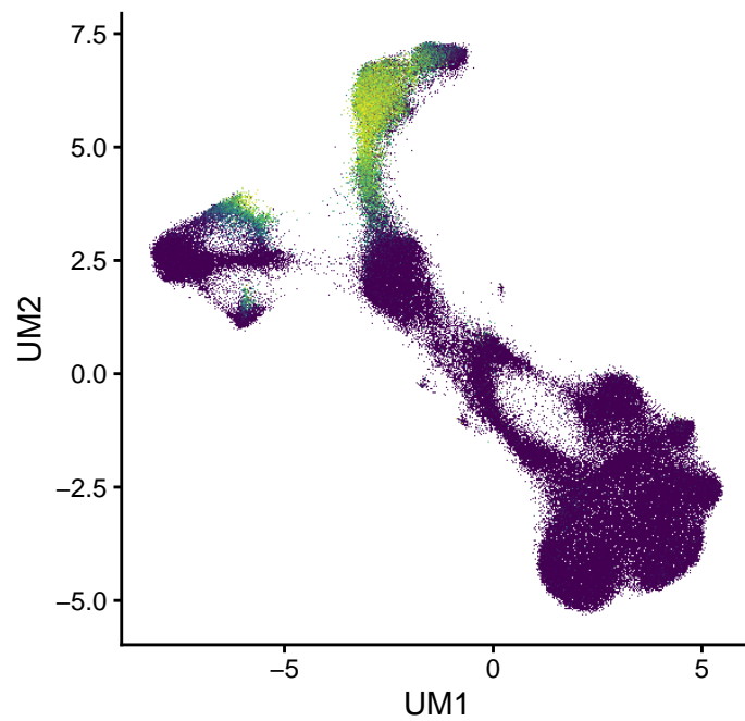
PECAM1 (0–4.6)
