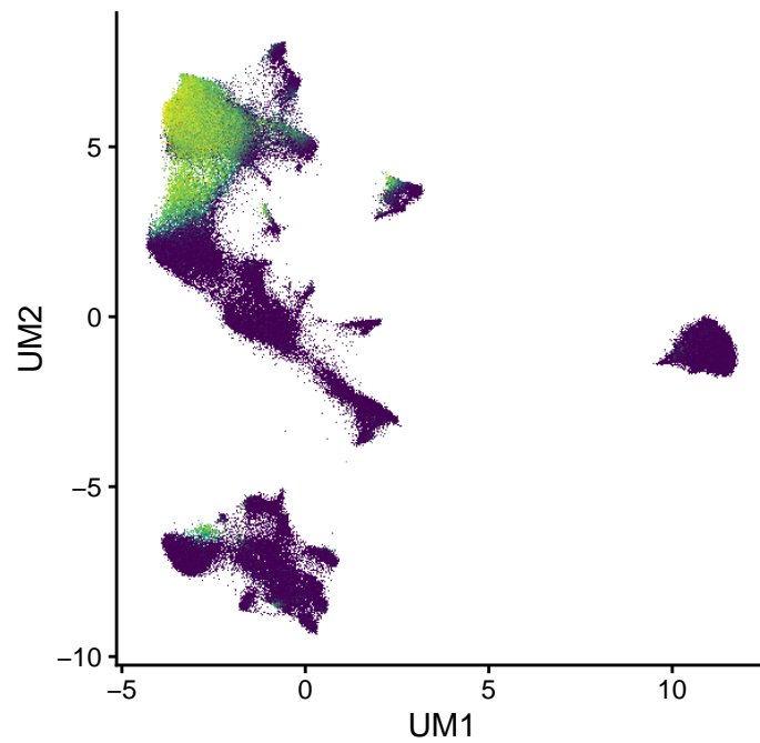
PECAM1 (0–4.7)
