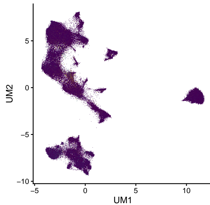
CD2 (0–3.6)
