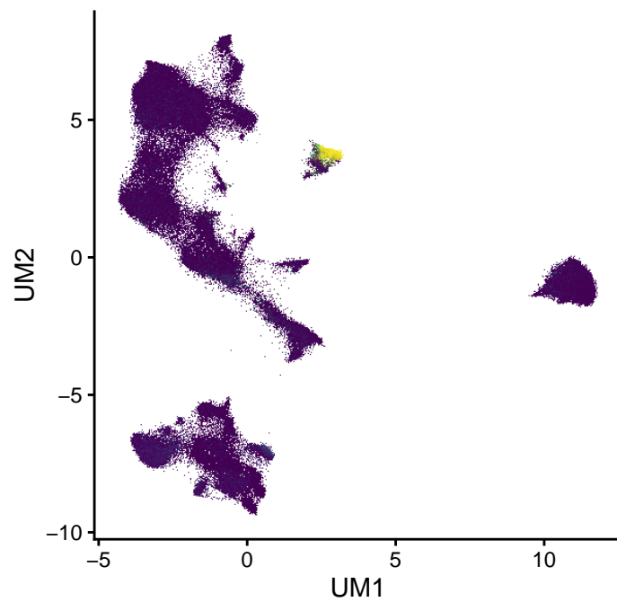
IGHG1 (0–8.2)
