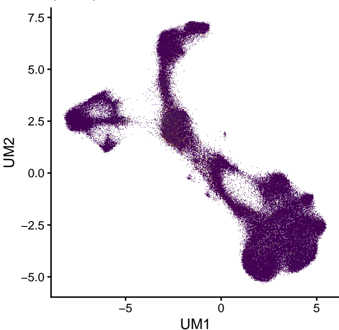
JCHAIN (0–2.7)
