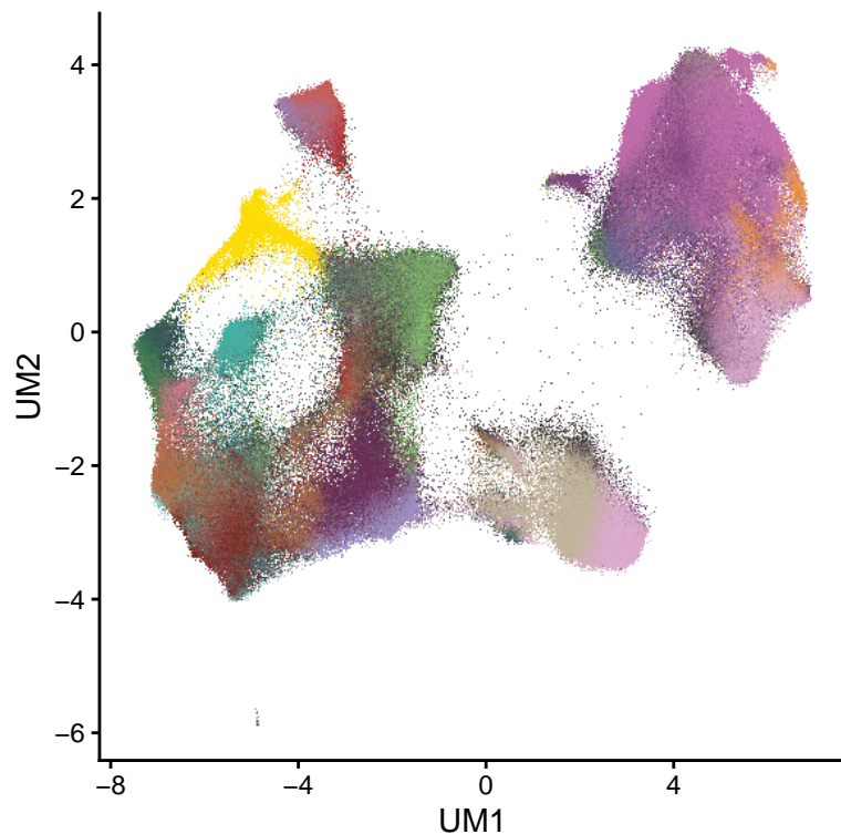
CRC: cell types (InSituType)
