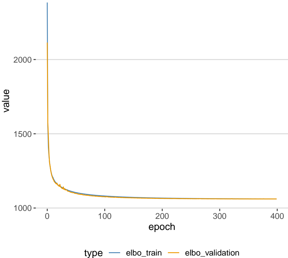
ELBO Plot for scVI Modeling
