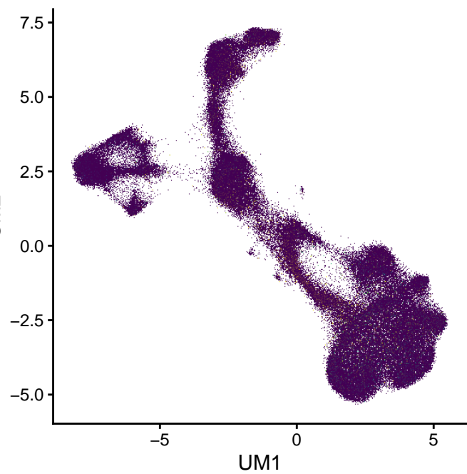
ELANE (0–4.3)
