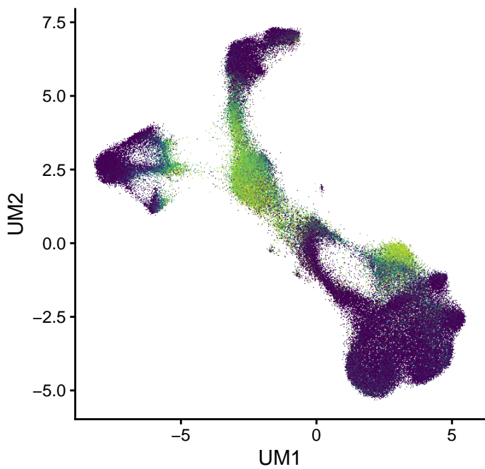
CD74 (0–7.2)
