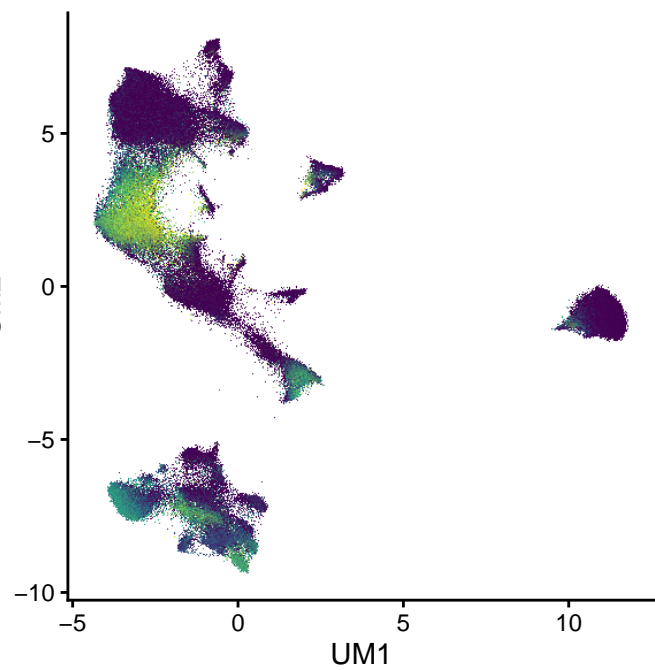
CD74 (0–6.6)
