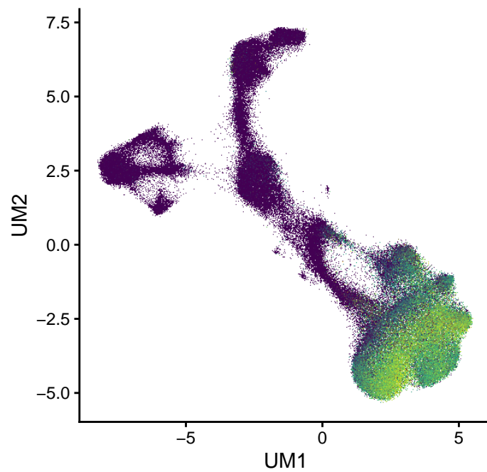
KRT19 (0–6.7)
