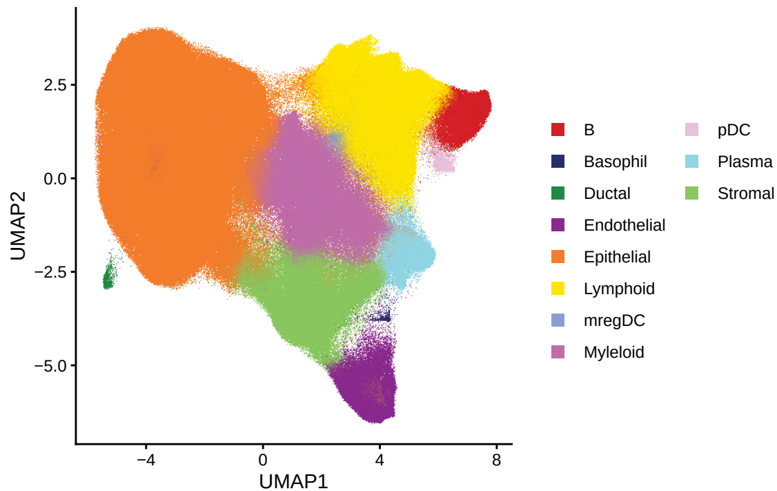
Cell Types (level 1)
