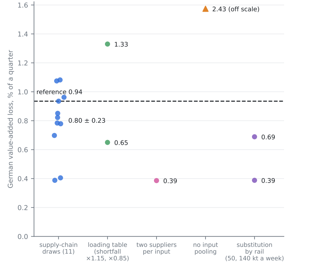
b 2018: sampling, structural and specification uncertainties, and the rules
