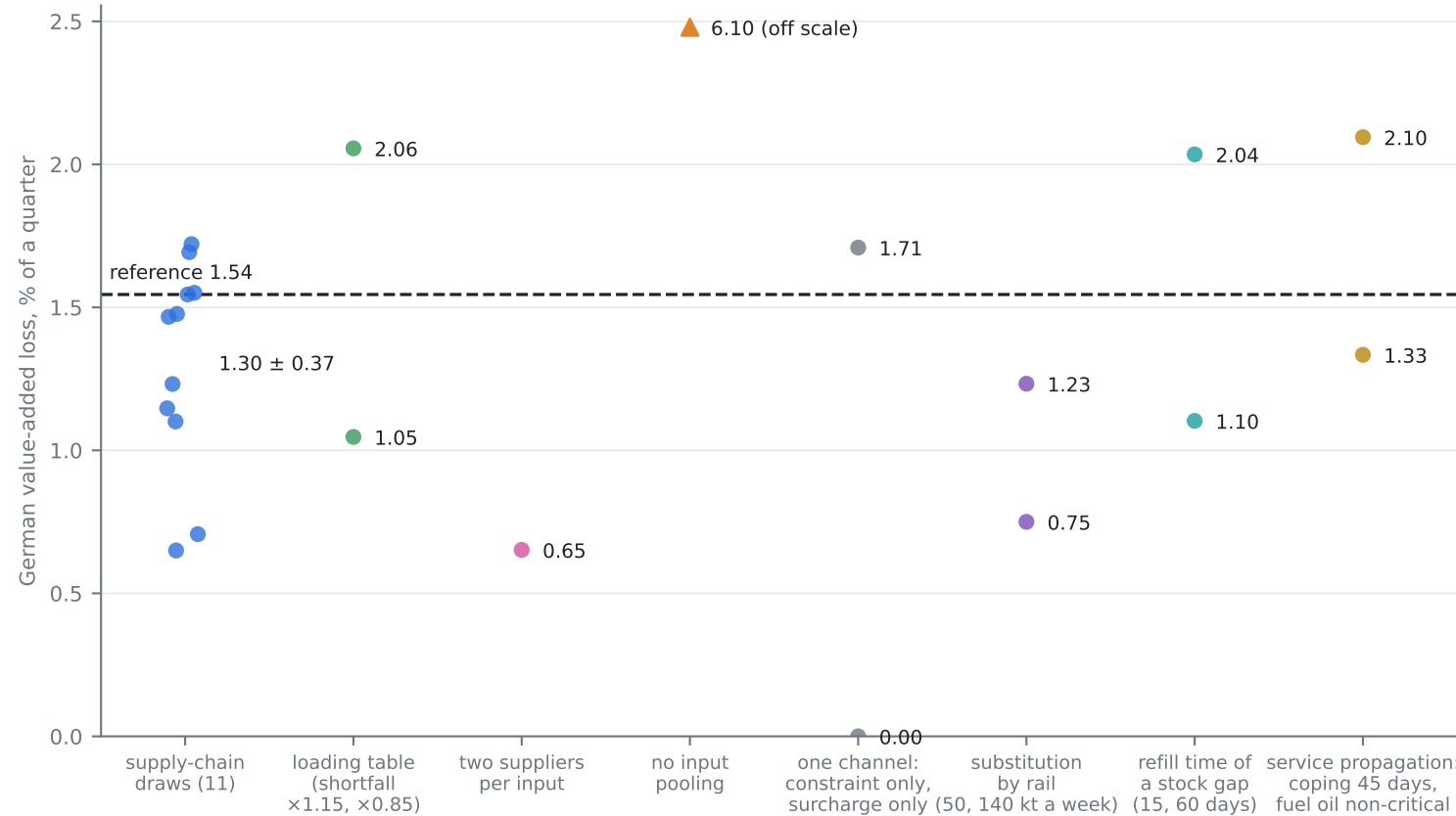
a 2026: sampling, structural and specification uncertainties, and the rules
