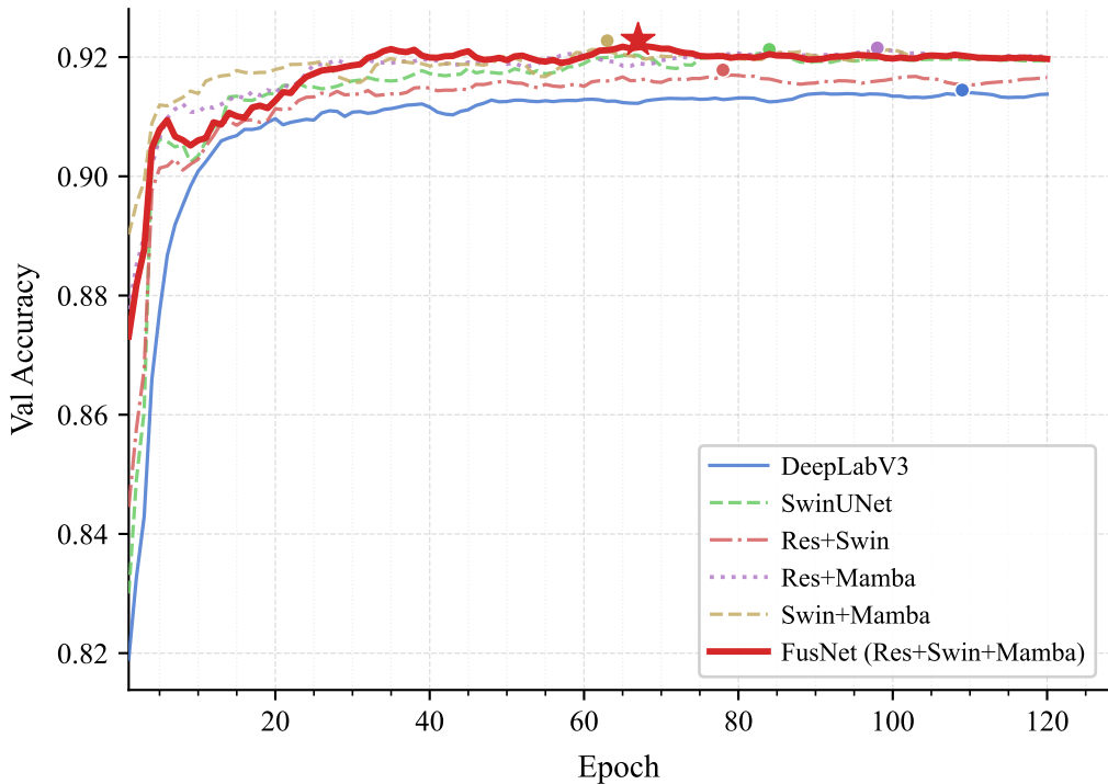
Validation Accuracy over Training Epochs
