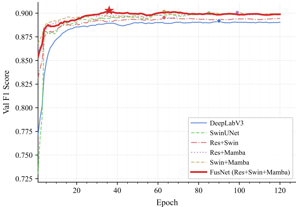
Validation F1 Score over Training Epochs
