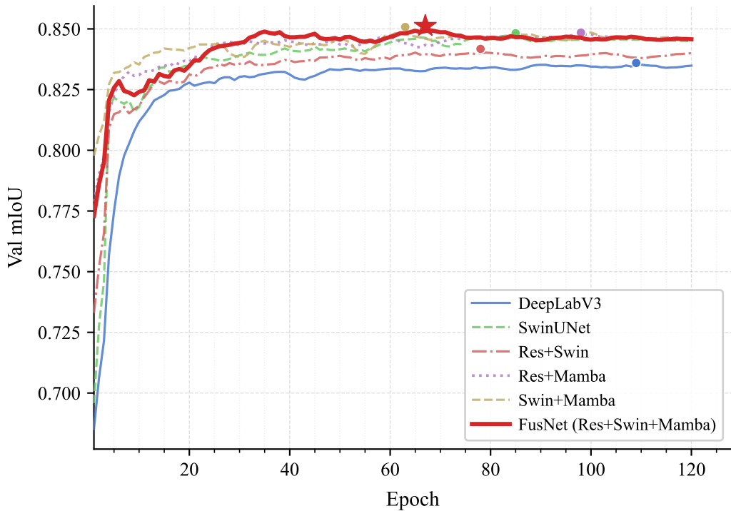
Validation mIoU over Training Epochs
