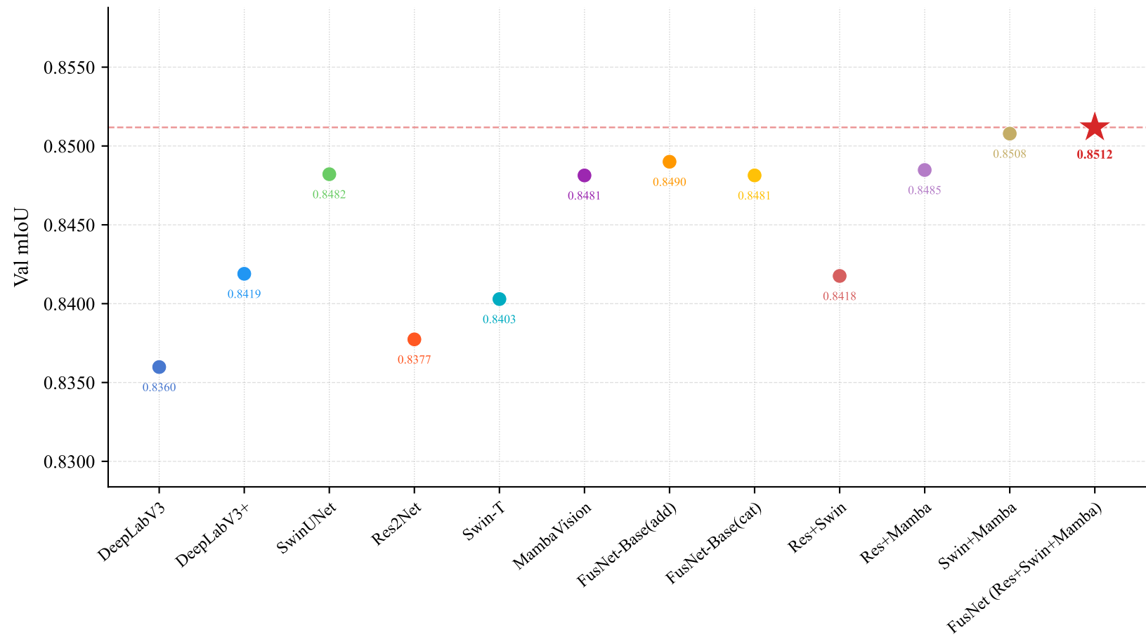
Val mIoU by Model
