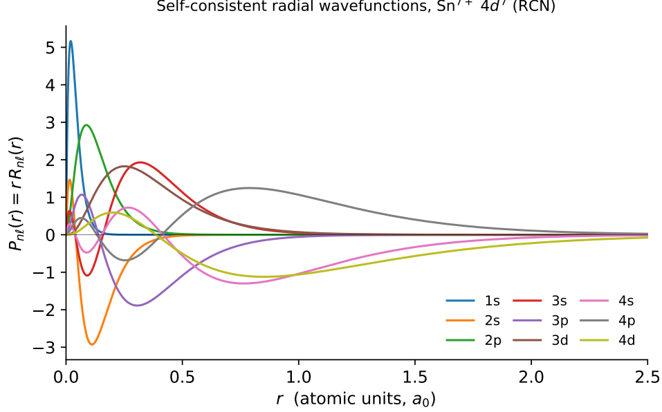
Figure 1: Self-consistent reduced radial wavefunctions P_{nl}(r) = r R_{nl}(r) for \text{Sn}^{7+} 4d^7 , computed by our build of RCN (the nine occupied subshells 1s through 4d). Each is normalized to \int P_{nl}^2 dr = 1 . This is real output of the engine, not a model.
