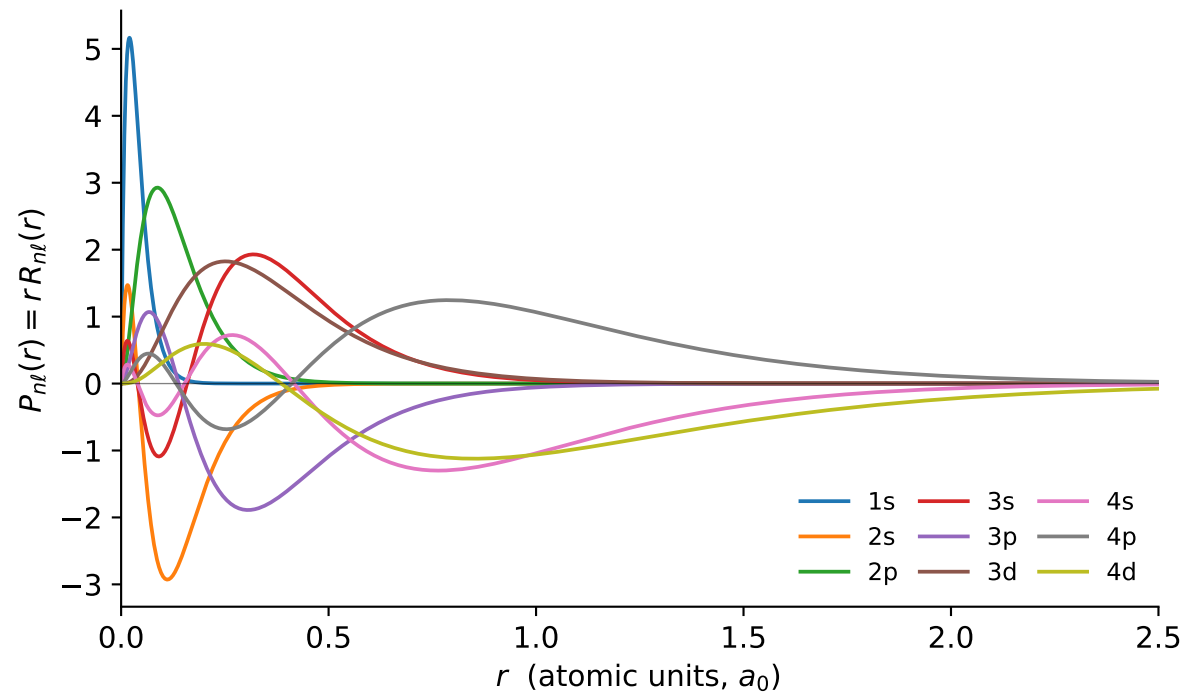
Self-consistent radial wavefunctions, \text{Sn}^{7+} 4d^7 (RCN)
