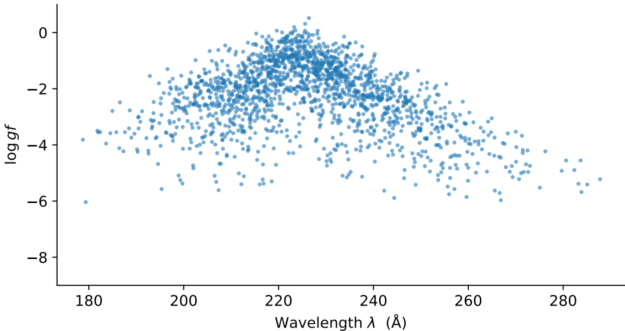
Computed E1 spectrum of \text{Sn}^{7+} : 4d^7-4d^65p (RCG)
