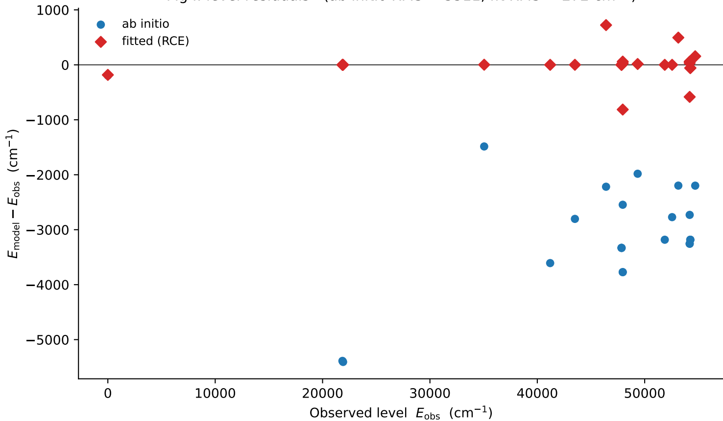
Mg I: level residuals (ab initio RMS = 3311, fit RMS = 272 cm -1 )
