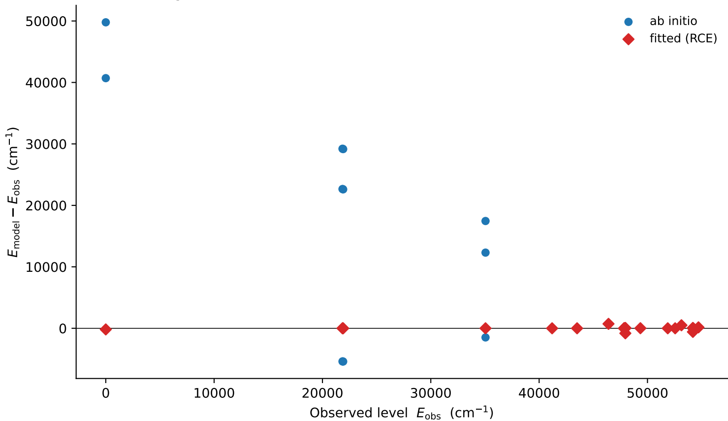
Mg I: level residuals (ab initio RMS = 24186, fit RMS = 272 cm -1 )
