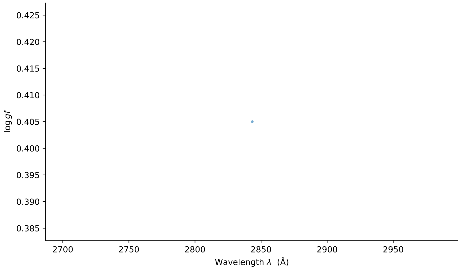
Mg I: computed E1 spectrum (1 lines)
