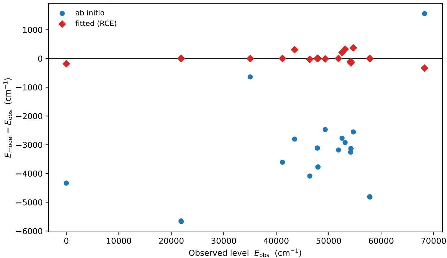
Mg I: level residuals (ab initio RMS = 3699, fit RMS = 147 cm -1 )
