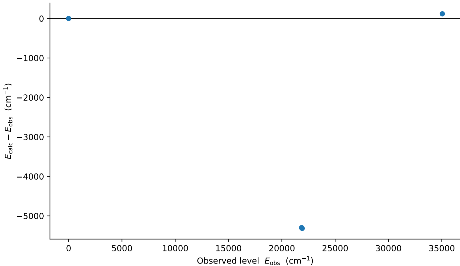
Mg I: level-fit residuals (RMS = 4111 cm -1 , ab initio)
