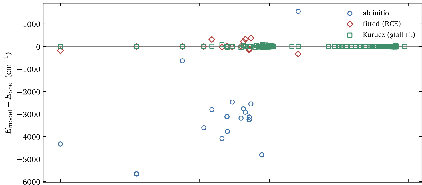
Mg I: level residuals (ab initio RMS = 3699, fitted RMS = 147, Kurucz RMS = 12 cm -1 )
