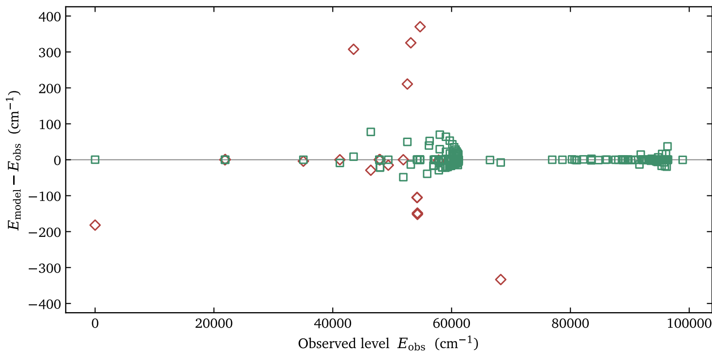
zoom to fitted residuals
