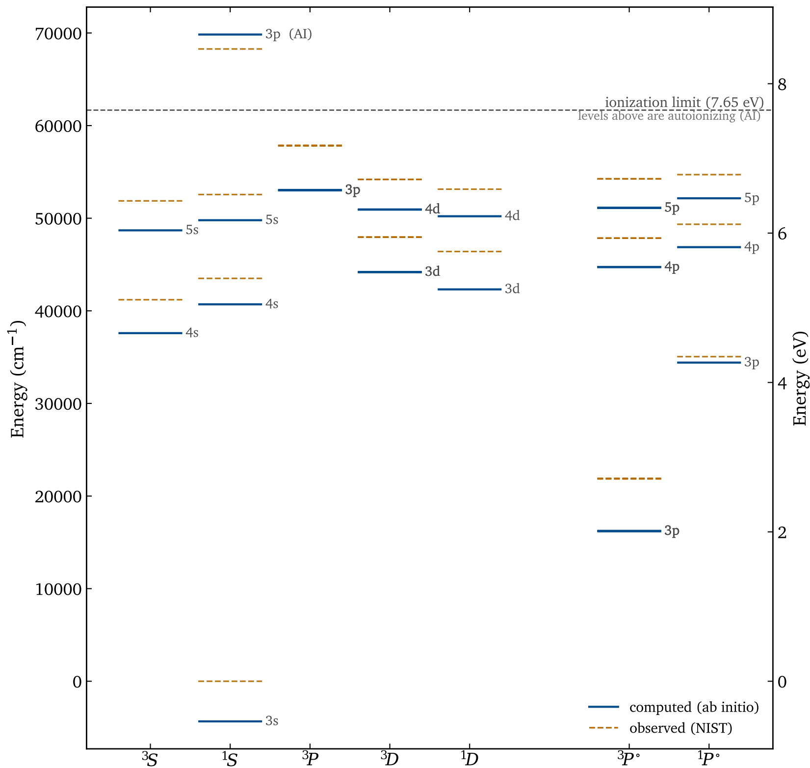
Mg I: term diagram - ab initio vs observed
