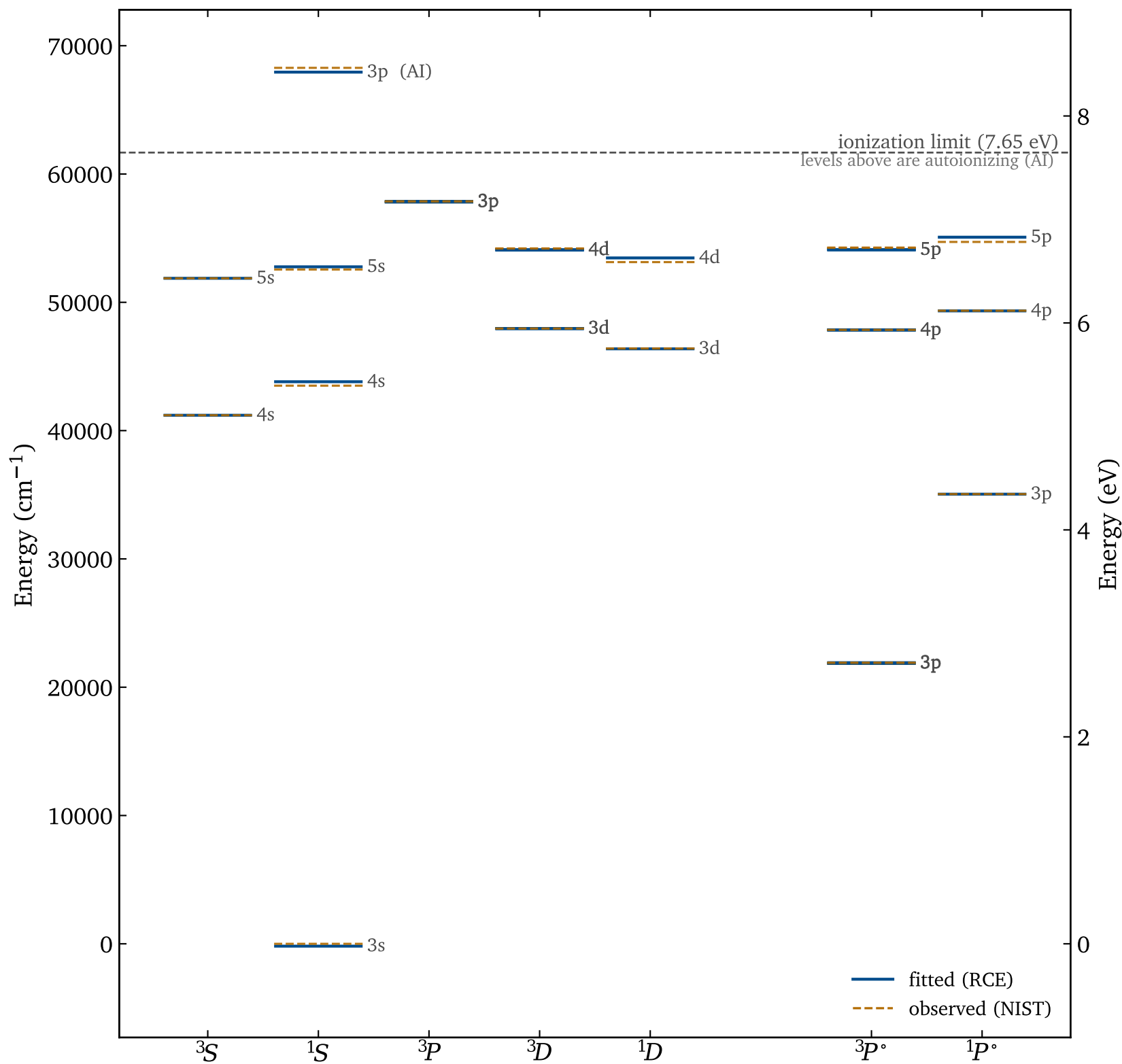
Mg I: term diagram - fitted vs observed
