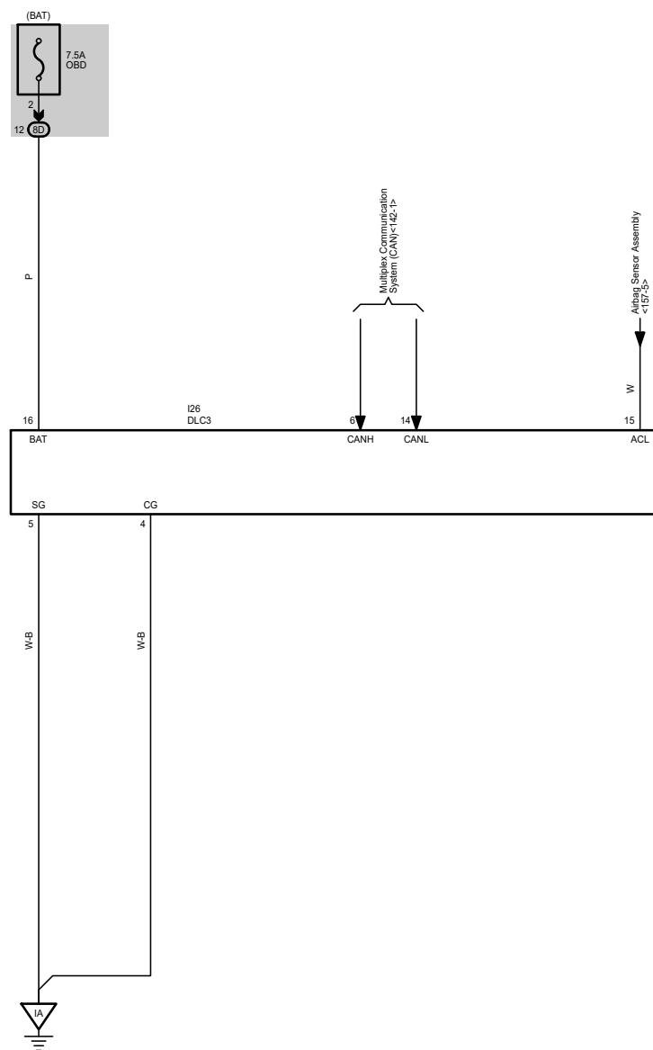
Data Link Connector 3 (G16E-GTS) (TMC Made H/B)
