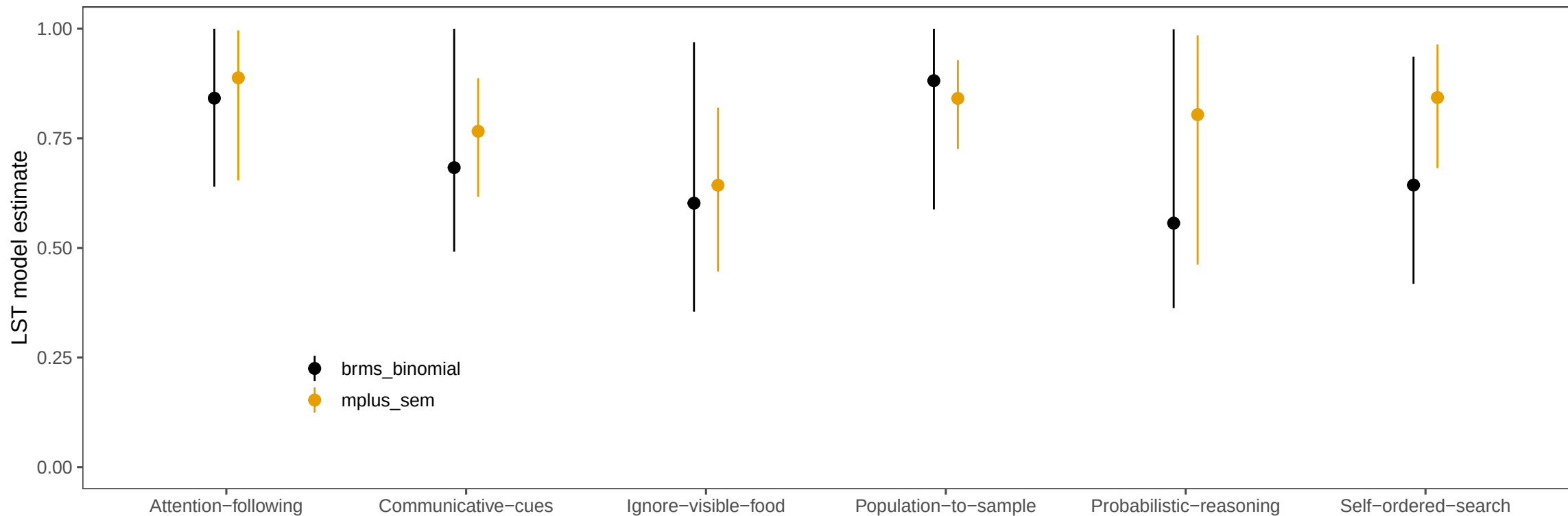
Consistencies across methods
