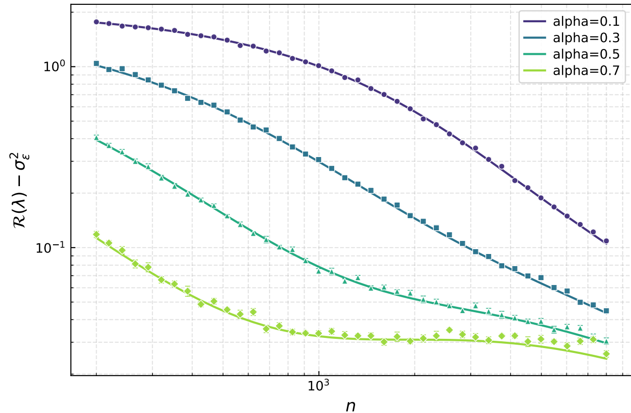
Fixed- \lambda NTK risk vs n ( p = 2000 )
