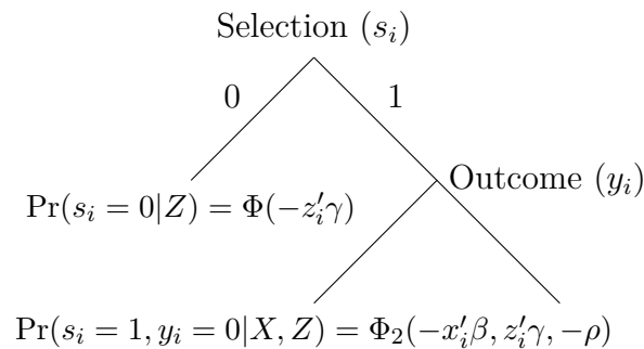
Figure 6.2: Visualizing the binary selection model
